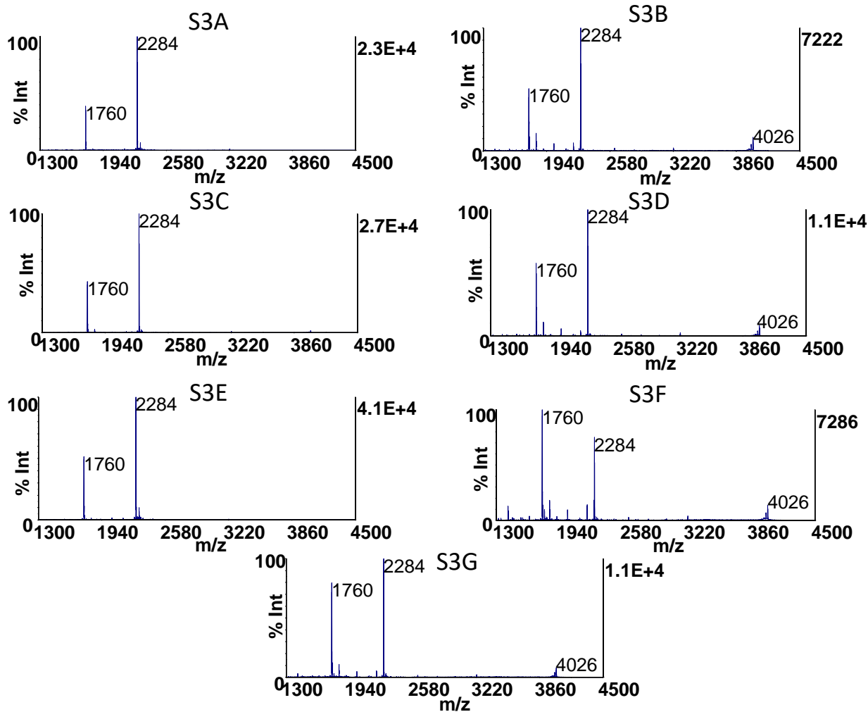
Supplementary Figure 3. Mass spectra from the reaction of Bval with BoNT/B1 (S3A), /B2 (S3B), /B3 (S3C), /B4 (S3D), /B5 (S3E), /B6 (S3F), and /B7 (S3G).
