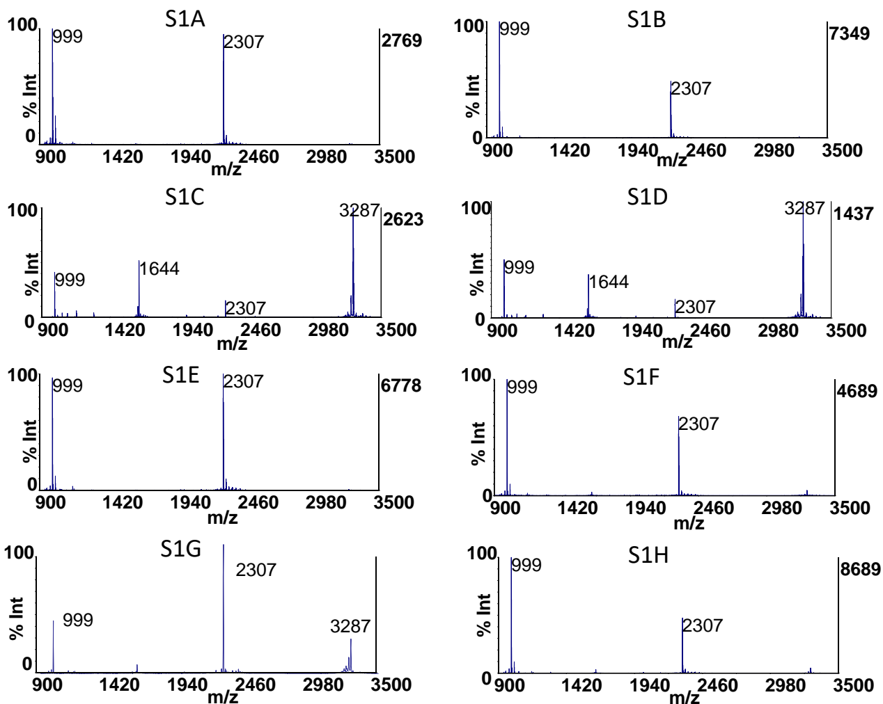
Supplementary Figure 1. Mass spectra from the reaction of Aval with BoNT/A1 (S1A), /A2 (S1B), /A3 (S1C), /A4 (S1D), /A5 (S1E), /A6 (S1F), /A7 (S1G), and /A8 (S1H)
