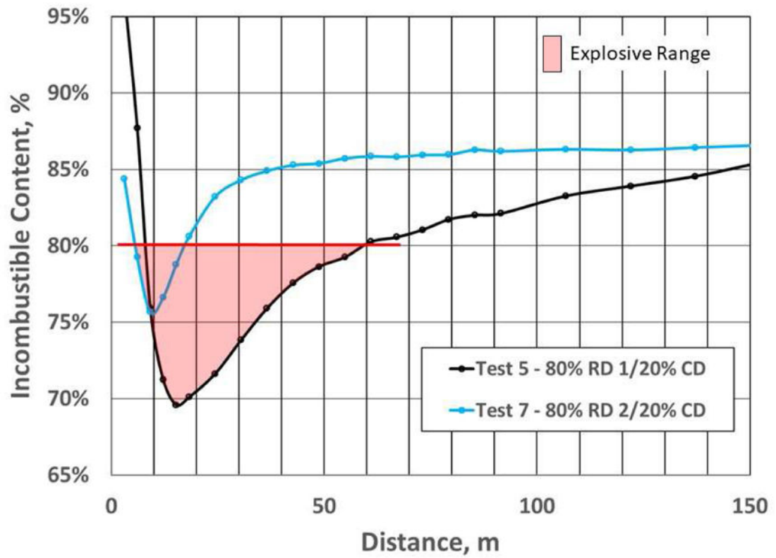
Figure 8. Comparison of the explosive zone lengths formed in Test 5 using RD 1 and Test 7 using RD 2. The red shaded area below 80% incombustible content indicates the explosive range
