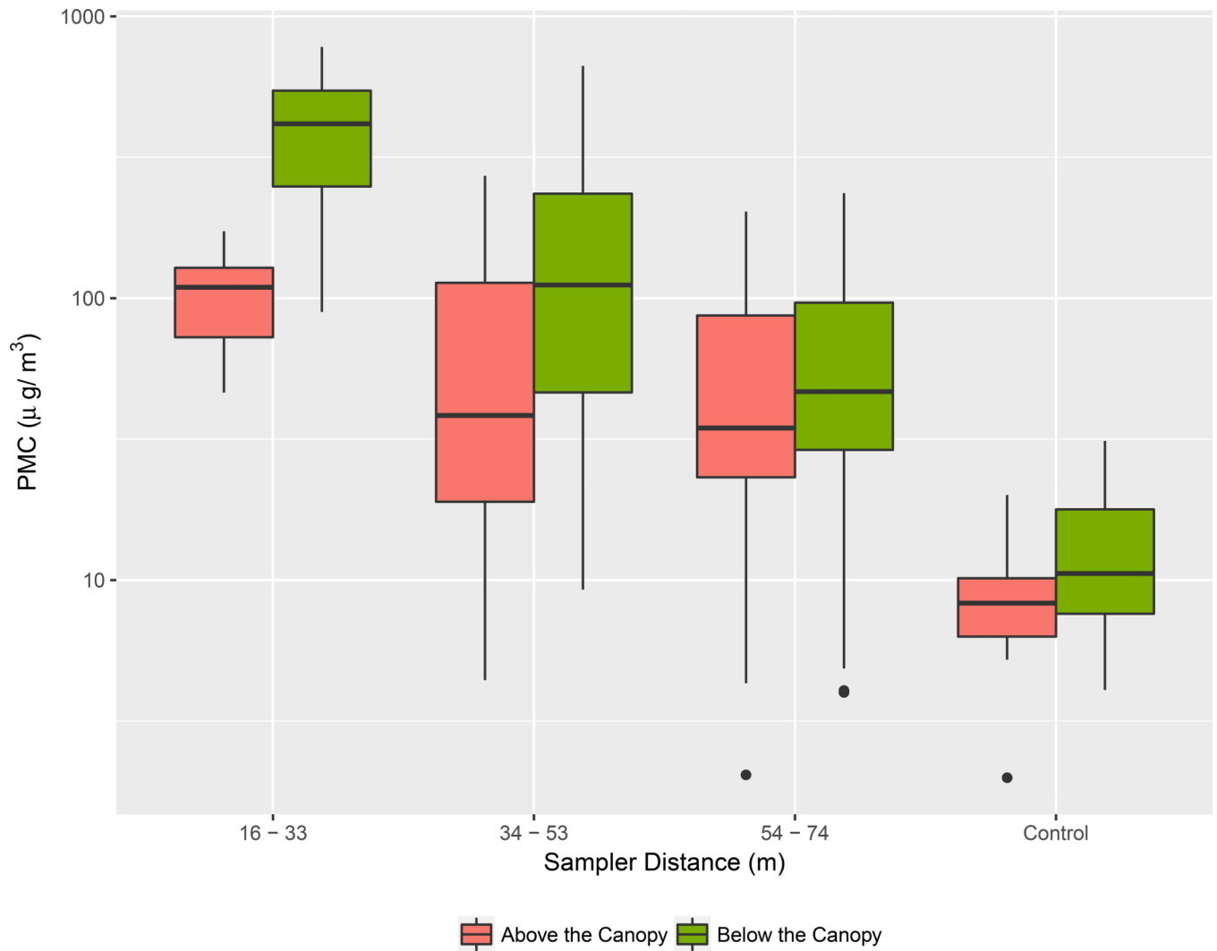
Figure 2. Boxplot using arithmetic mean PMC levels ( \mu\text{g}/\text{m}^3 ) above and below the canopy at increasing distances from the central proximal edge of the spray quadrant. PMC is on the log scale.
