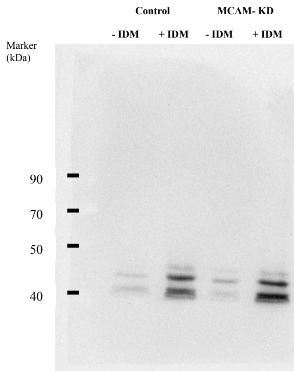
Fig 6C. Phospho ERK1/2
