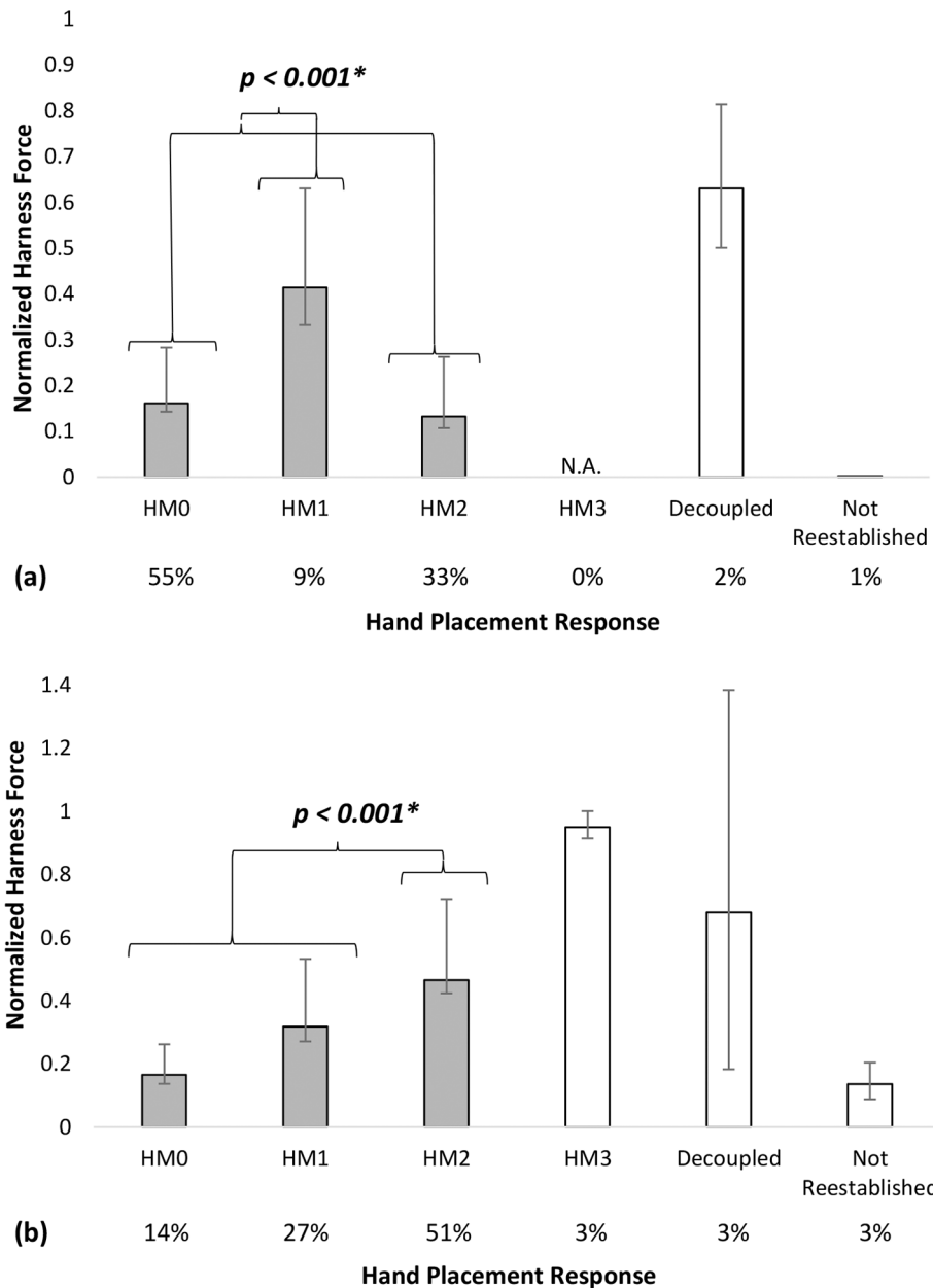
Figure 2: Average normalized harness force across hand placement responses during a) ascending and b) descending perturbations. Standard deviation of normalized harness force is represented by the positive error bars and standard error of normalized harness force is represented by the negative error bars. Occurrence (percentage) of each hand placement response is displayed on the horizontal axis below each hand placement response label. Note statistical analysis was not performed for trials where the hand moved three rungs (HM3), decoupled from the rung (decoupled), or left the rung, but did not reestablish hand contact prior to end of perturbation response (hand not reestablished) (white bars). N.A. indicates that no data was recorded for that condition.
