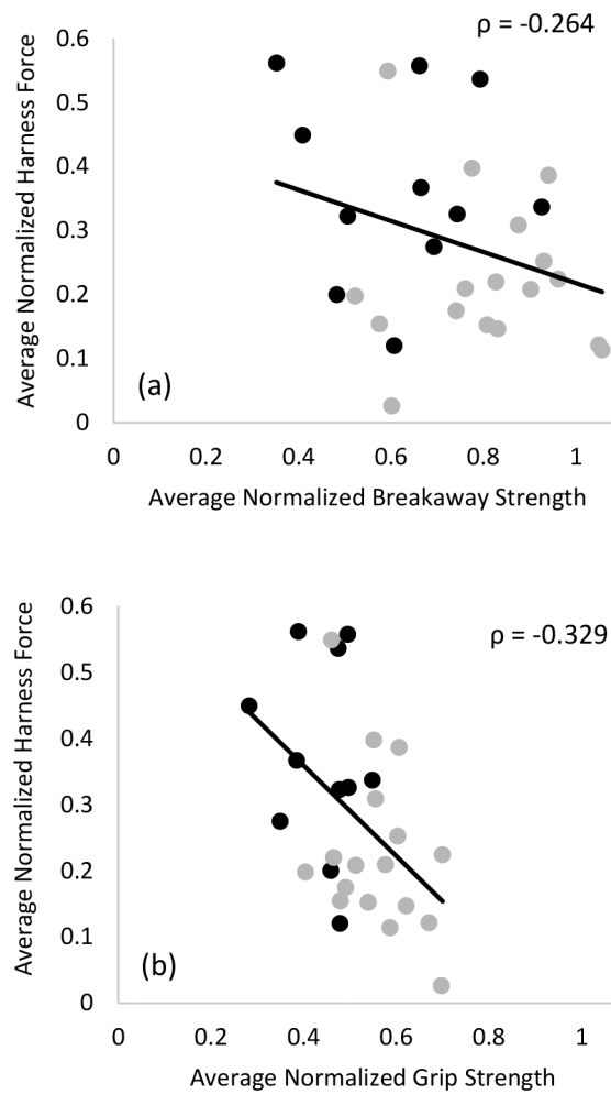
Figure 4: Relationship between the average normalized harness force with a) breakaway strength and b) grip strength. Each dot represents a person's average normalized harness force across all six perturbations. Male participants are represented by the gray dots and female participants are represented by the solid darker dots. The solid line represents the best linear fit. Spearman's correlations ( \rho ) are displayed on each graph.
