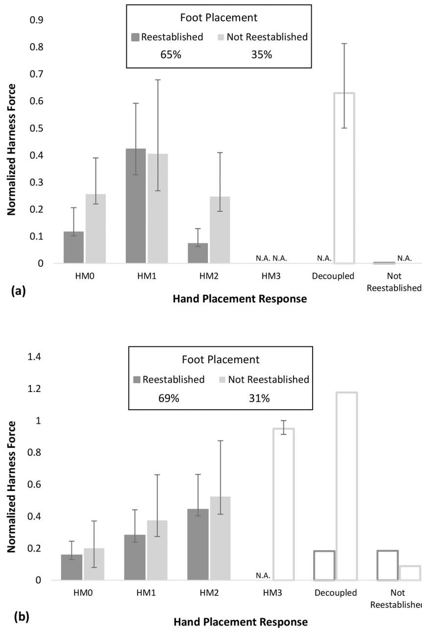
Figure 3: Average normalized harness force for hand and foot placement combinations after a) ascending and b) descending perturbations. Certain hand placement outcomes were not included in the statistical analyses including HM3, decoupled or hand not reestablished (outlined bars). Standard deviation of normalized harness force is represented by the positive error bars and standard error of normalized harness force is represented by the negative error bars. Data elements, where the foot reestablished contact, are represented by the dark gray bars and data elements, where the foot did not reestablish contact, are represented by the light gray bars. Occurrence (percentage) of each foot placement response is displayed under
