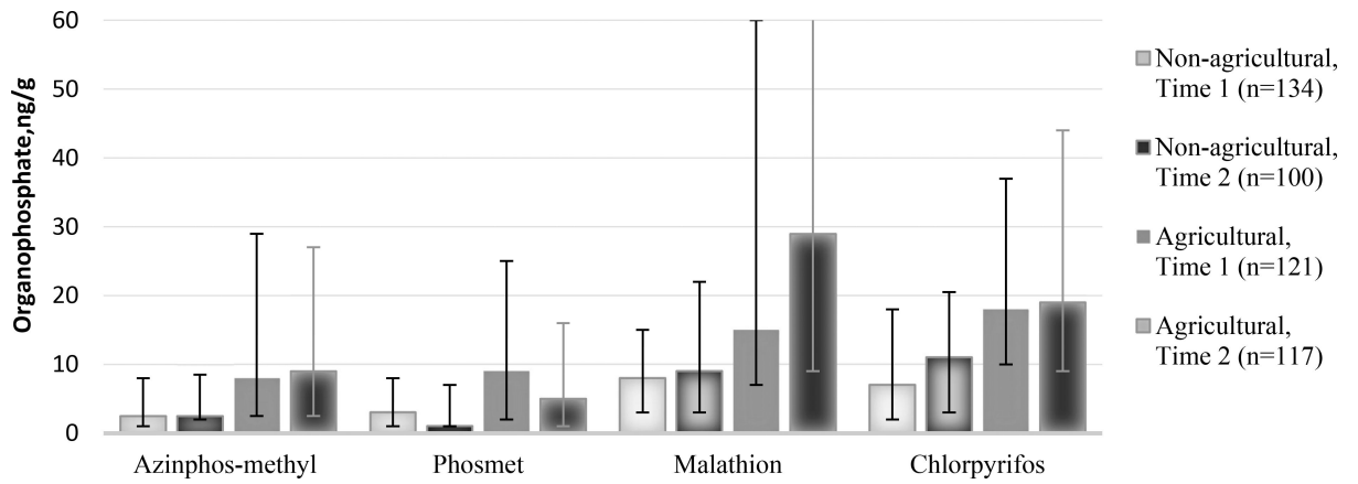
Figure 2. Median organophosphate concentrations and interquartile ranges in carpet dust samples from non-agricultural and agricultural households at Time 1 and Time 2 (2008–2011). Note: 75 th percentile for malathion in agricultural households at Time 2= 110 ng/g dust.
