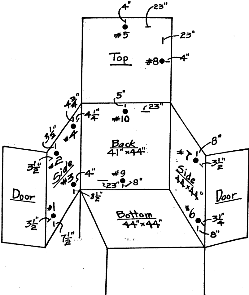
FIGURE 4.—Thermometer locations.
