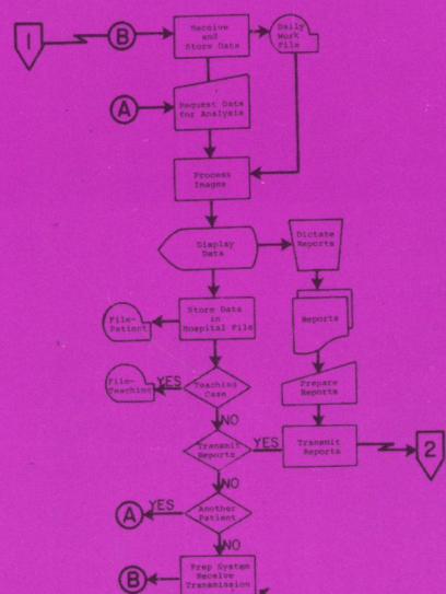
System Flowchart for Central Analysis Station
