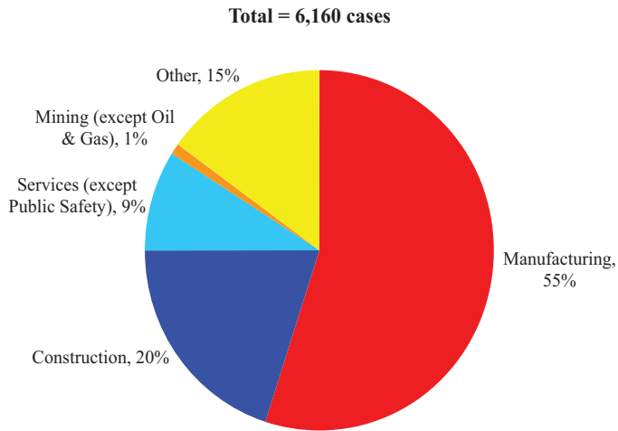
36a. Distribution of workers with BLLs \geq 10 \mu\text{g}/\text{dL} , by industry, 2016 (18 states)
