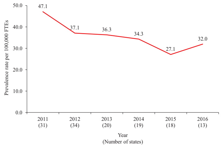
36b. Prevalence rate of workers with BLLs \geq 10 \mu\text{g}/\text{dL} in construction, 2011-2016
