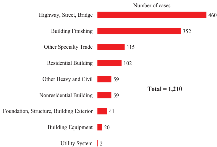
36c. Number of workers with BLLs \geq 10 \mu\text{g}/\text{dL} , by construction subsector, 2016 (13 states)
