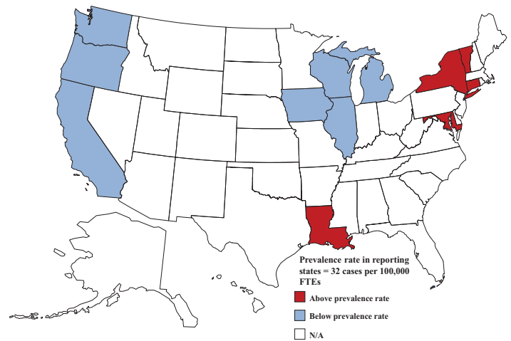
36d. Prevalence rate of construction workers with BLLs \geq 10 \mu\text{g}/\text{dL} , by state, 2016 (12 states)
