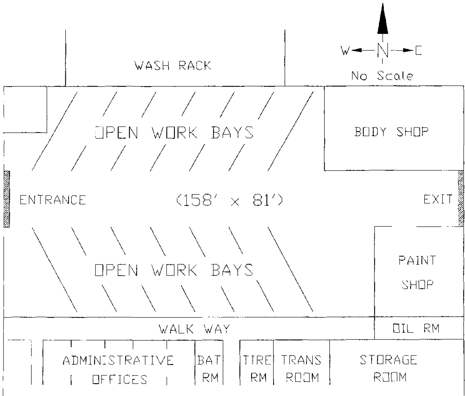
Figure 4-4. Layout of garage with enclosure B.
