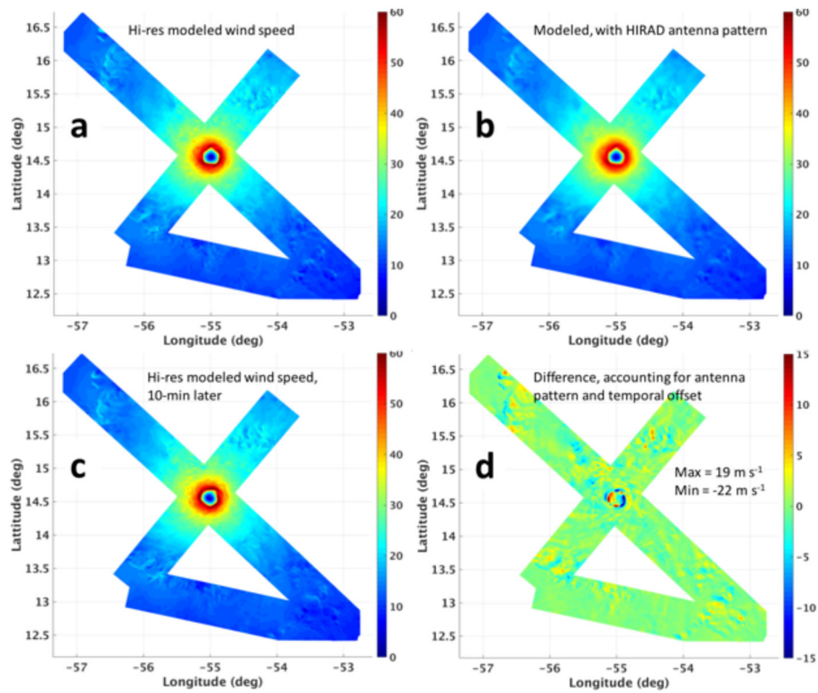
Figure 7. (a) Surface wind speed ( \text{m s}^{-1} ) for a 1-km resolution idealized numerical model, with a hypothetical aircraft figure-4 pattern applied. (b) As in (a), but smoothed with HIRAD's antenna pattern. (c) As in (a), but 10 minutes later to simulate conditions encountered by dropsondes. (d) The difference (b) – (c).
