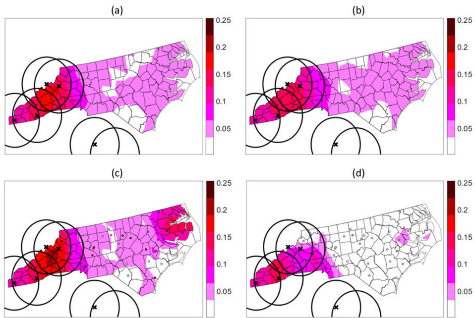
Figure 1. Map of benzo(b)fluoranthrene ( ng/m^3 ). Maps of mean benzo(b)fluoranthrene concentration for North Carolina on April 16, 2005 across the 4 prediction methods: (a) kriging, (b) cokriging, (c) Linear Regression BME, (d) log-Mass Fraction BME. Square markers indicate observed data, circle markers indicate PAH estimates, X's mark known fires for that day with a 100 km buffer.
