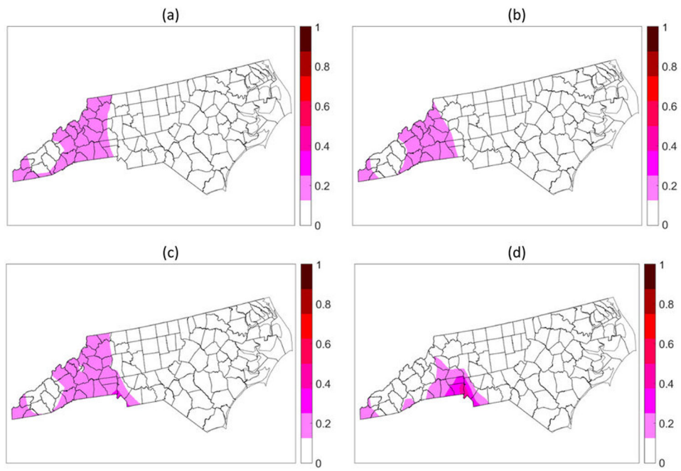
Figure 2. Probability of exceedance. Probability of annual benzo(a)pyrene exceeding 0.25 \text{ ng/m}^3 across North Carolina in 2005 as predicted by (a) kriging, (b) cokriging, (c) Linear Regression BME and (d) log-Mass Fraction BME.
