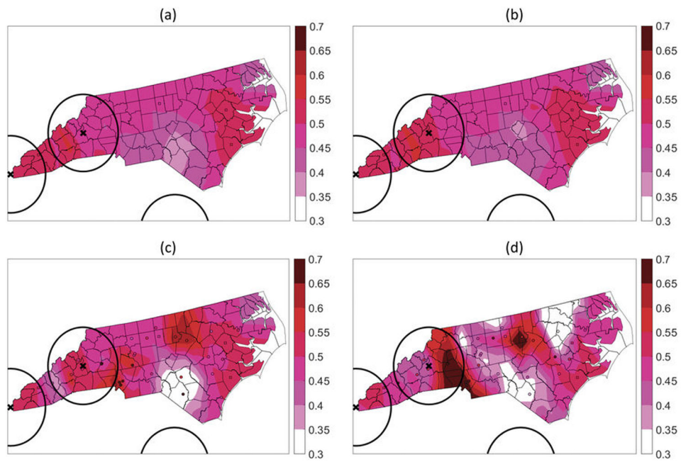
Figure 3. PAH ratios. Ratio of indeno(1,2,3-c,d)pyrene/(indeno(1,2,3-c,d)pyrene +benzo(g,h,i)perylene) on March 5, 2005 in North Carolina across the 4 prediction methods: (a) kriging, (b) cokriging, (c) Linear Regression BME, (d) log-Mass Fraction BME. Square markers indicate the ratio of observed data, circle markers indicate the ratio of PAH estimates, X's mark known fires for that day with a 100 km buffer.
