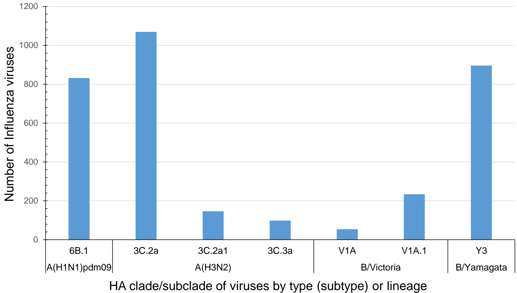
SUPPLEMENTARY FIGURE 3. Genetic characterization of viruses — United States, October 1, 2017– May 19, 2018*
