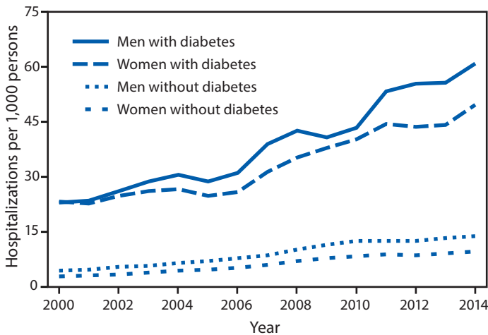
FIGURE 1. Age-standardized incidence* of hospitalizations with acute kidney injury† among men and women aged ≥20 years with and without diabetes — United States, 2000–2014
