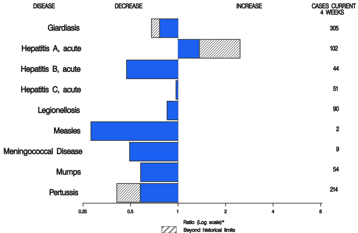
FIGURE I. Selected notifiable disease reports, United States, comparison of provisional 4-week totals March 10, 2018, with historical data
