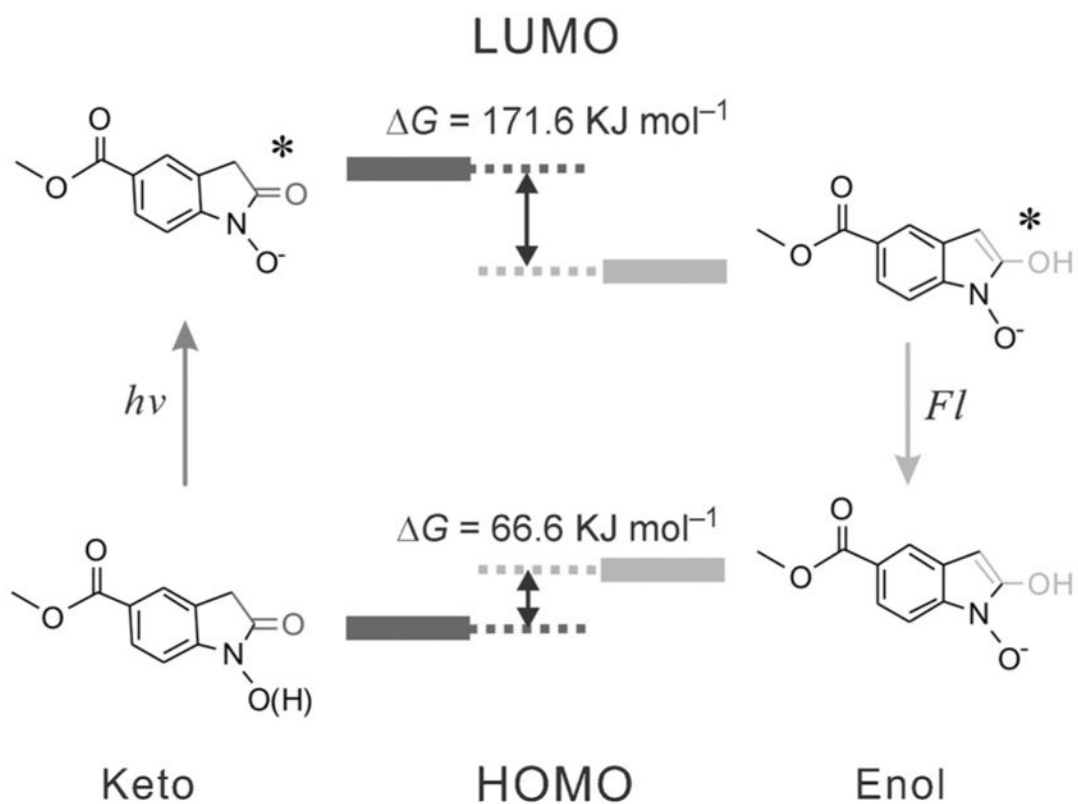
Figure 3. Schematic illustration of the proposed excited-state keto–enol tautomerization of 1 a , whereas only the enol form is the fluorescent moiety. HOMO and LUMO calculations of the keto and enol forms computed by DFT calculations show that enol form of 1 a is more stable at the excited state than the keto form.
