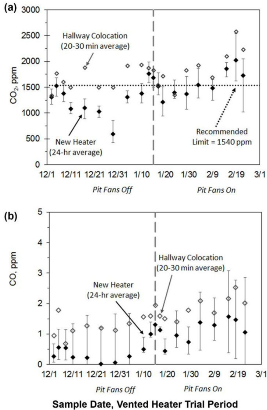
Figure 6. Average (a) CO 2 and (b) CO concentrations from the second winter (cyclone + vented heater testing), averaged over all monitors, including hallway collocation data. Error bars for 24 h data represent data ranges. Vertical dashed lines indicate the date when manure pit fans were activated.
