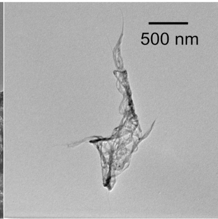
b. Small CNT clusters found from ESPnano tube after sonication of CNT coating solution.
