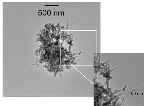
d. CNT airborne particles collected by ESPnano during the probe sonication process at source.
