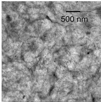
c. Fiber structured CNTs found from CNT dip coating solution after sonication.
