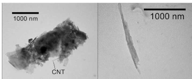
g. CNT airborne particles mixed with other particle collected at PBZ.
