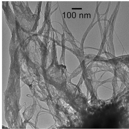
a. Large CNT clusters found from ESPnano tube after sonication of CNT coating solution.
