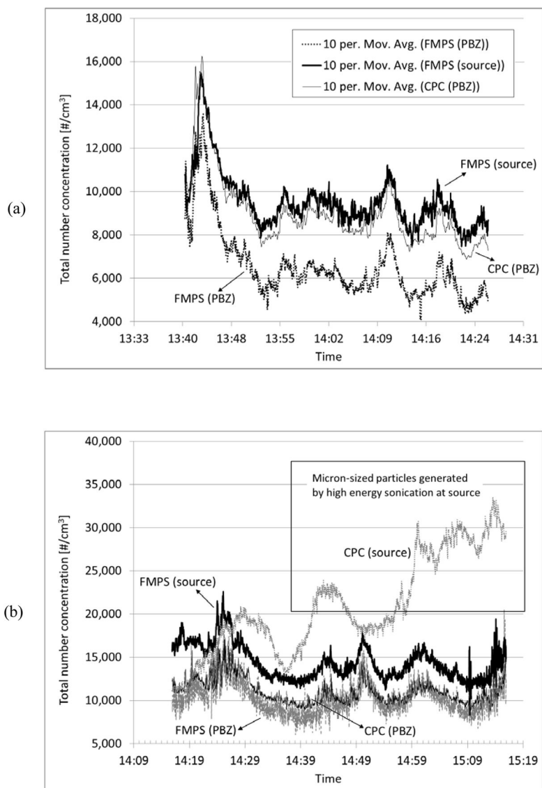
Figure 1. Task of probe sonication process monitored with the FMPSs and CPCs for (a) Solution A, and (b) Solution B. Moving average trendlines were used in Figure 1a to provide a clearer view of concentration changes.
