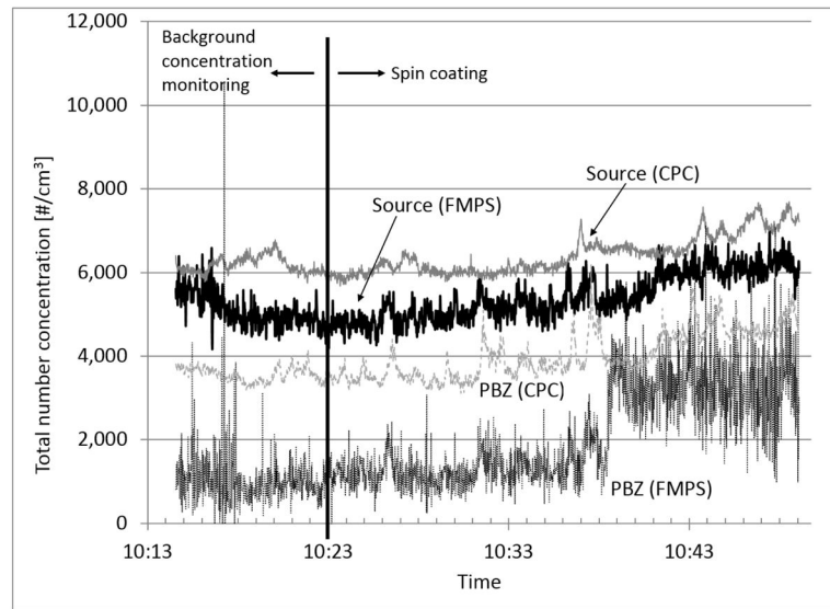
Figure 4. Real-time monitoring data for the spin coating process.
