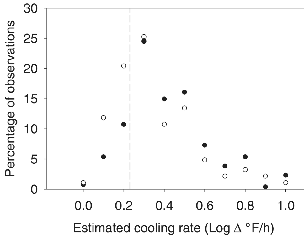
Figure 4. Effect of food depth on estimated cooling rate. Cooling rates for food in shallow pans ( 3 in. [7.6 cm] deep) indicated by closed circles; cooling rates for food in deep pans (>3 in. [7.6 cm] deep) indicated by open circles. Food Code cooling rate is 0.23 (cooling to 41°F [5°C] within 6 h), indicated by the dotted vertical line.
