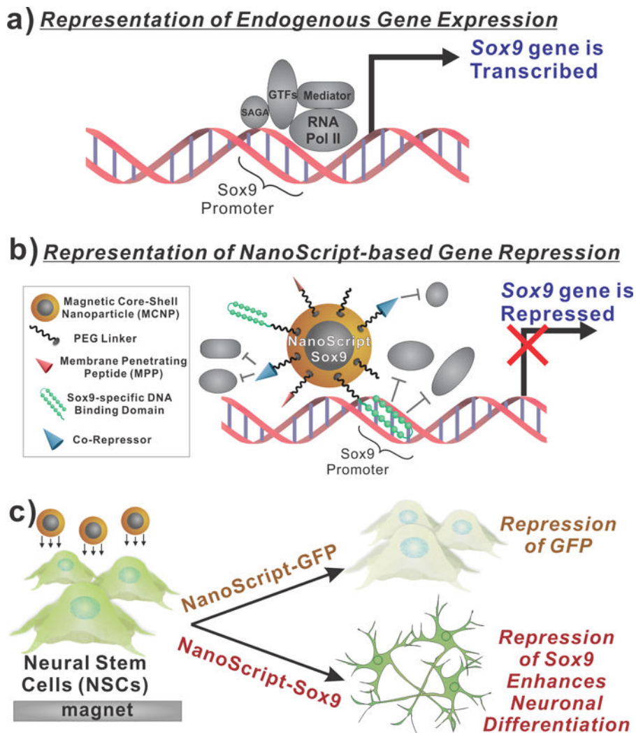
Figure 1. Schematic Representation of NanoScript-based Gene Repression
