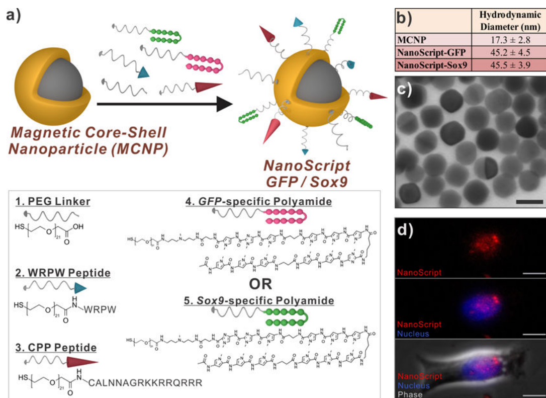
Figure 2. Construction and Characterization of NanoScript
