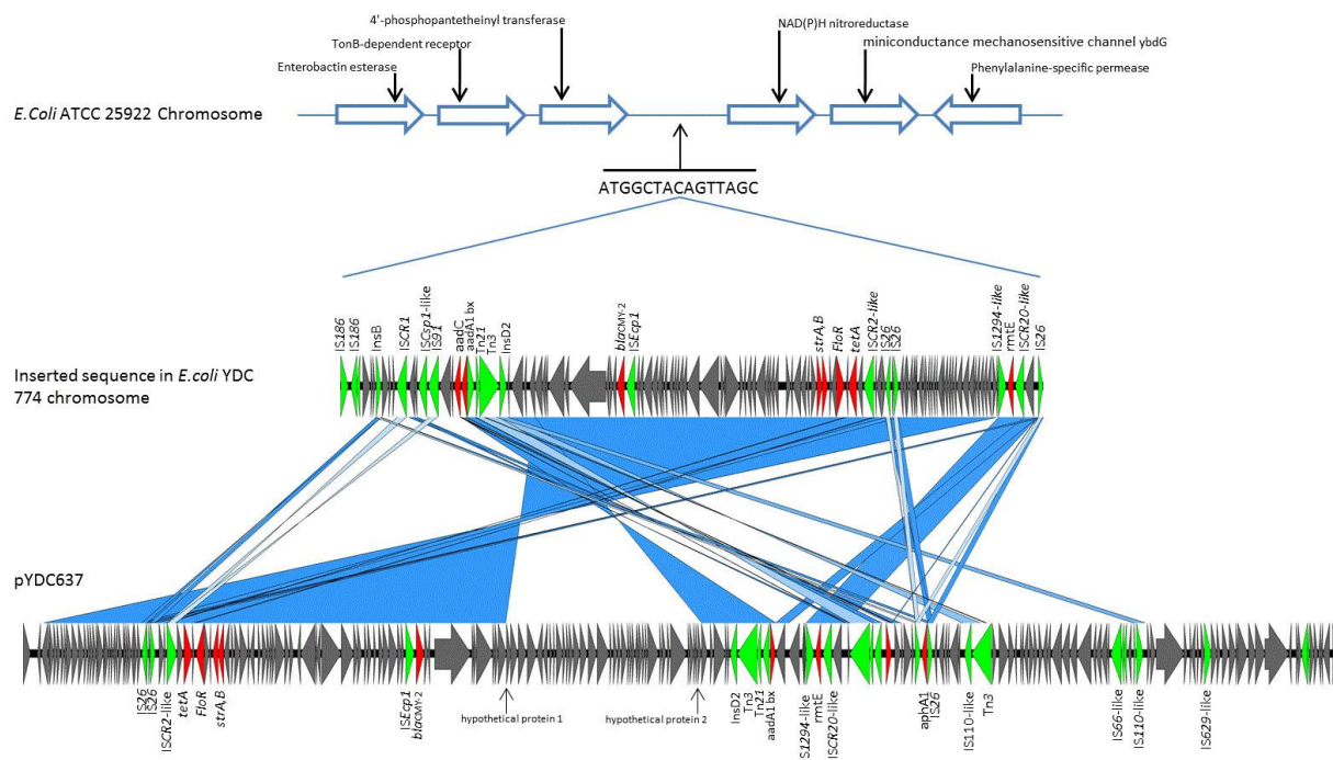
Technical Appendix Figure. Comparative analysis of the rmtE1 -carrying region of the chromosome of Escherichia coli YDC774 (GenBank accession number no. MIGD00000000.0) and pYDC637 (GenBank accession no. KP056256) from E. coli YDC637. Red arrows indicate antimicrobial resistance genes. Green arrows indicate mobile elements. Gray arrows indicate other genes. ST, sequence type.
