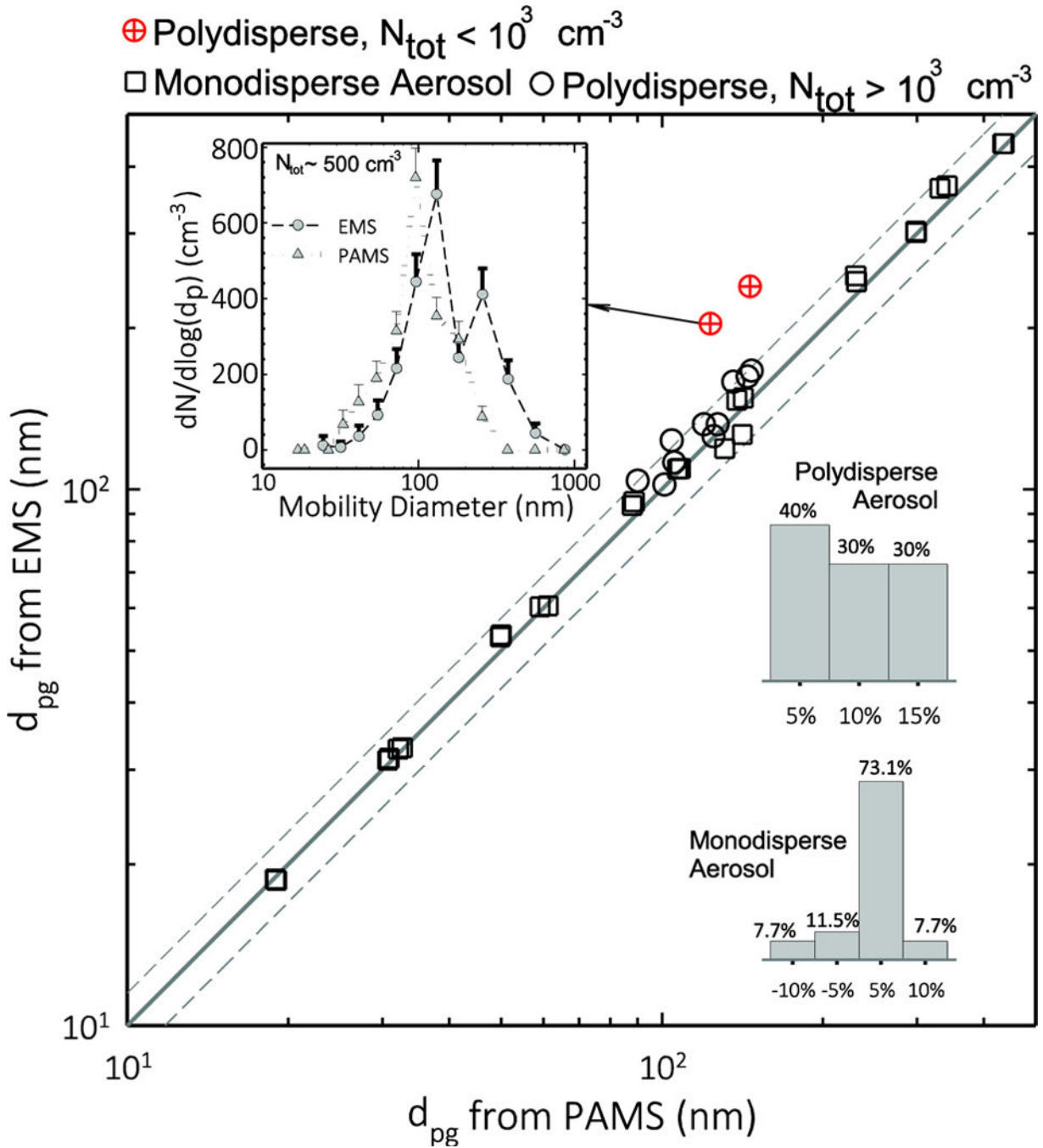
Figure 2. Comparison of sizing accuracy of PAMS and EMS at identical mobility resolution for near-monodisperse and polydisperse aerosols. The inset histograms show percent of samples tested (on y-axis), for each monodisperse and polydisperse aerosol, as a function of percent difference in measured d_{pg} from the two instruments (i.e. (d_{pg}^{EMS} - d_{pg}^{PAMS}) / d_{pg}^{EMS} ).
