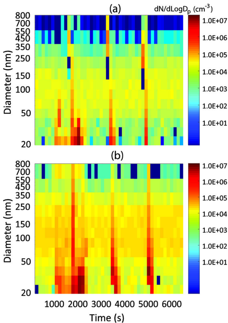
Figure 5. Time series comparison of particle size distribution of (a) PAMS and (b) SMPS™. Combustion aerosol from a propane flame was used as the test aerosol, and was moved in and out of the sampling zone of the two instruments to mimic transient samples.
