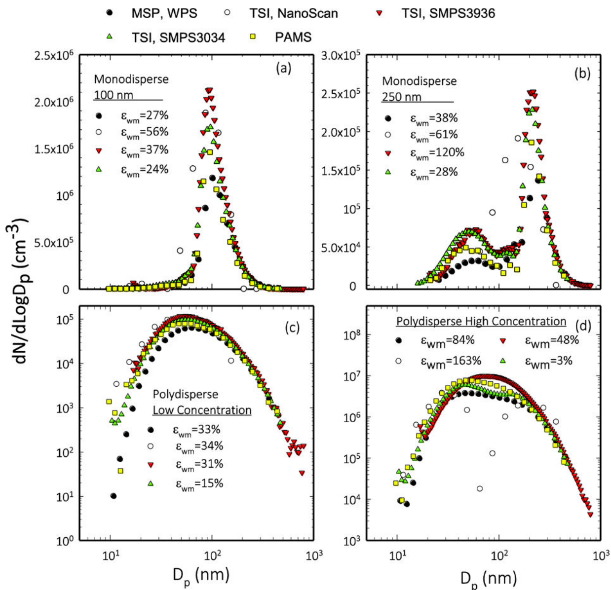
Figure 3. Comparison of particle size distributions of monodisperse and polydisperse aerosol obtained from PAMS with that from various commercial spectrometers. \epsilon_{wm} was computed using Equation (2).
