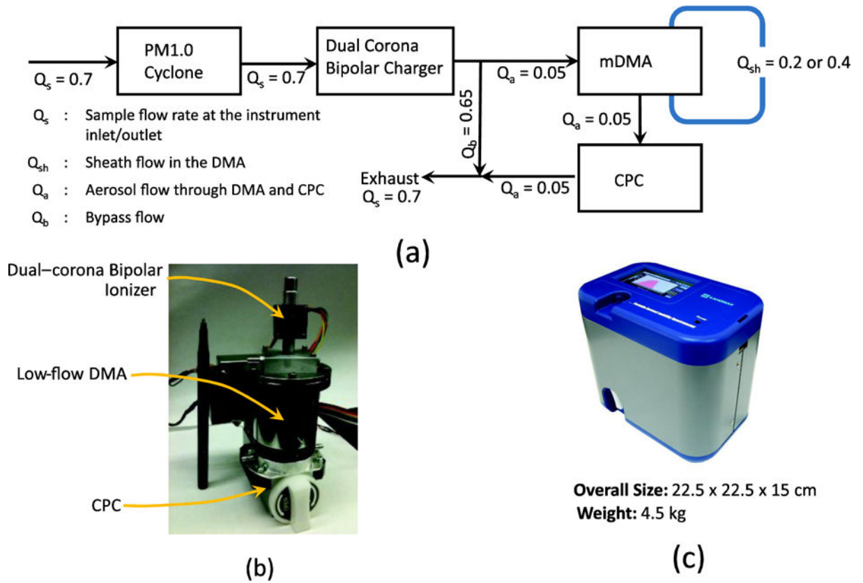
Figure 1. (a) Flow scheme and layout of different components of PAMS; (b) assembly of charger, DMA, and CPC units; (c) prototype PAMS instrument
