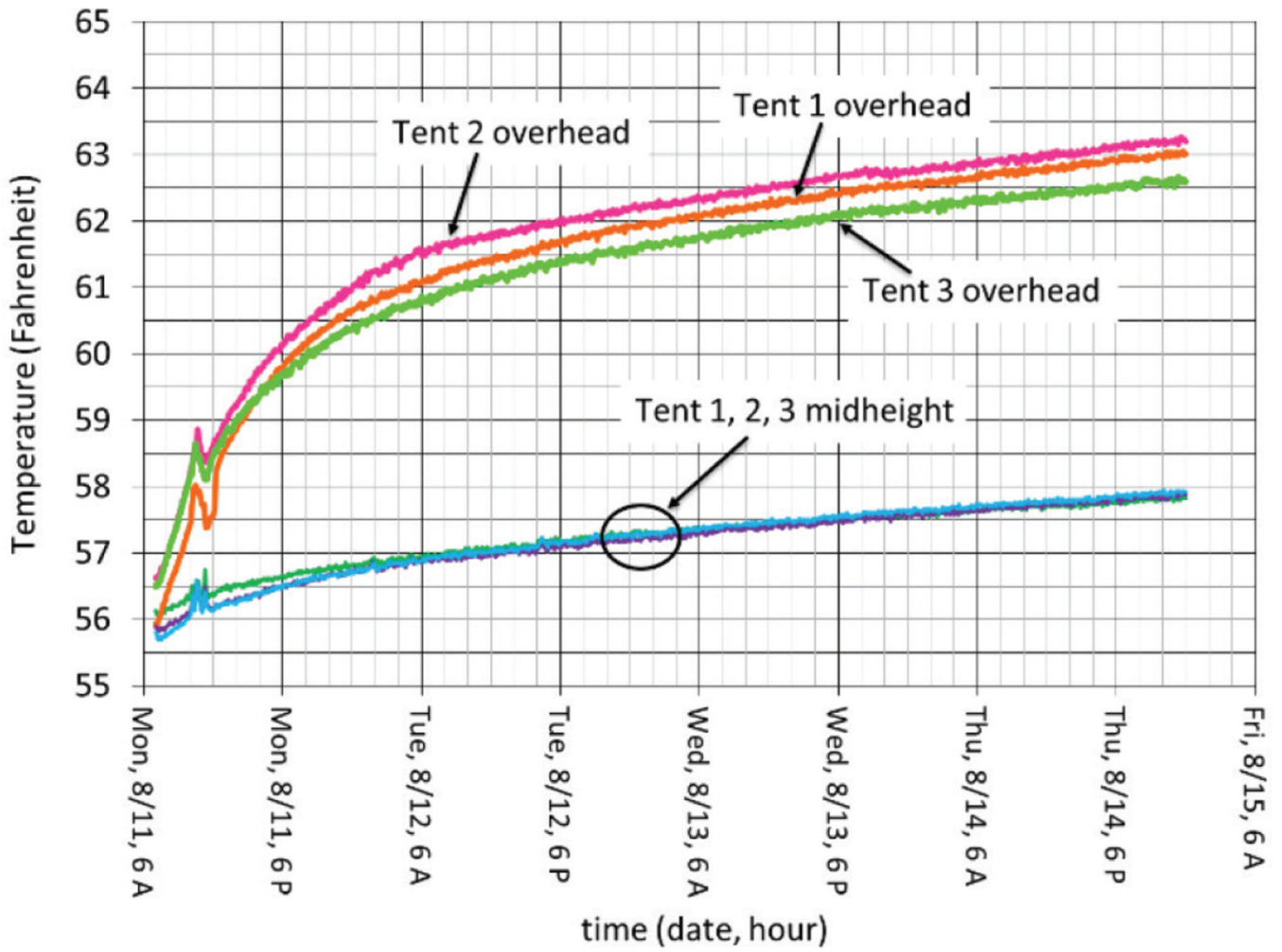
Figure 5. Mine air temperature along the sides of the RA at mid-height and over the tent.
