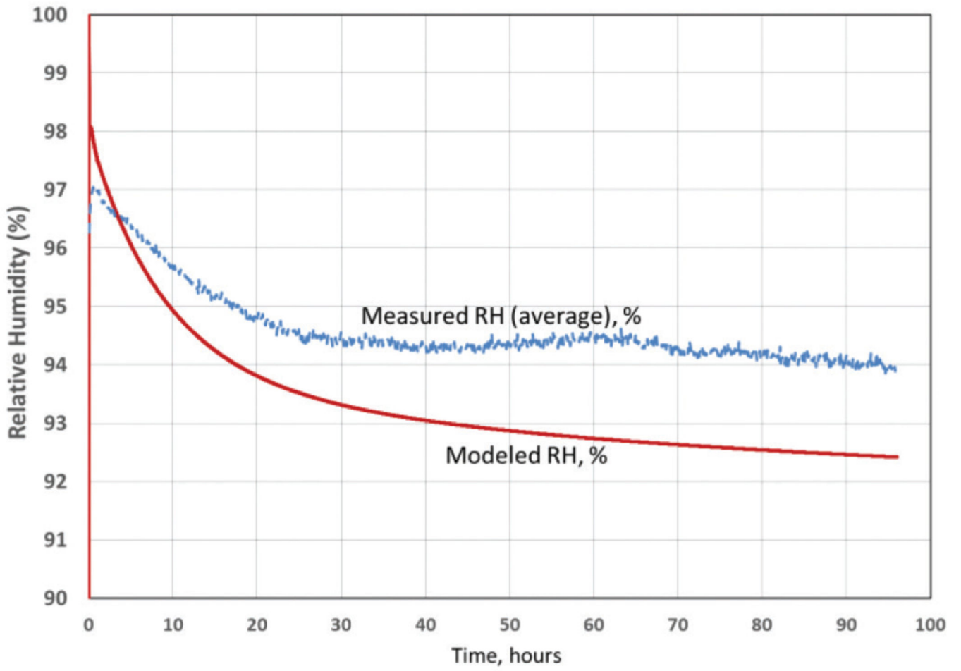
Figure 8. Modeled (solid line) versus measured (dotted line) interior relative humidities.
