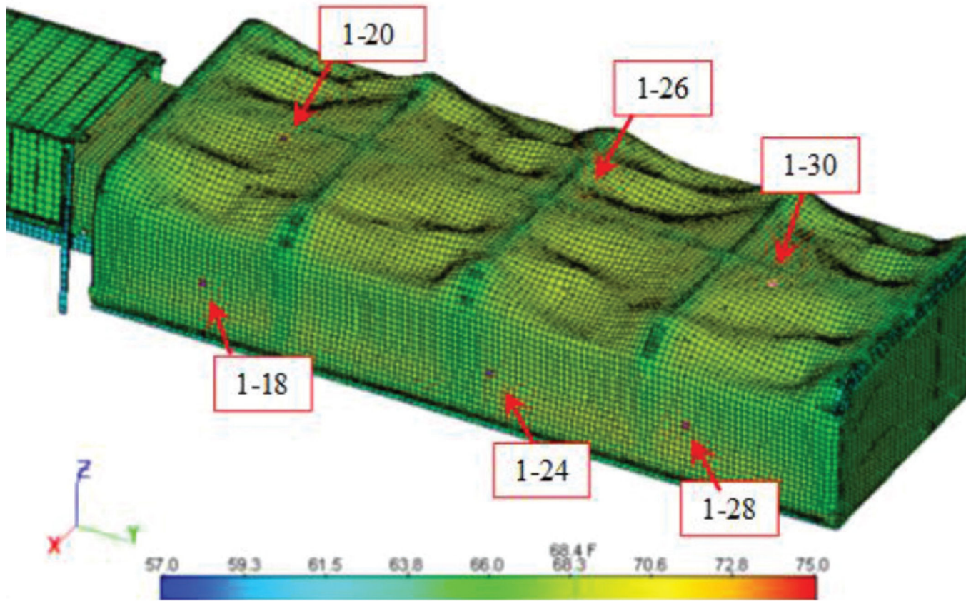
Figure 9. Three-dimensional view of the simulated RA model at the end of the 96-hour test.
