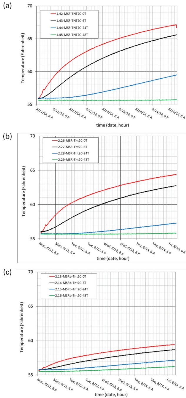
Figure 6. Mine strata temperatures for: (a) floor under the center of Tent 2, (b) roof above the center of Tent 2 and (c) rib at the center of Tent 2, as measured during the 96-hour test.
