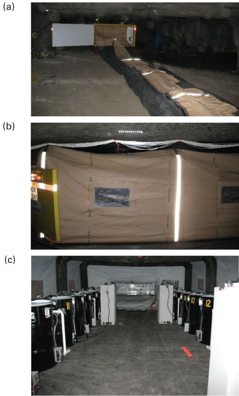
Figure 1. A 23-person tent-type RA: (a) during deployment, (b) after deployment and (c) showing an interior view with simulated miners and heated water tanks.
