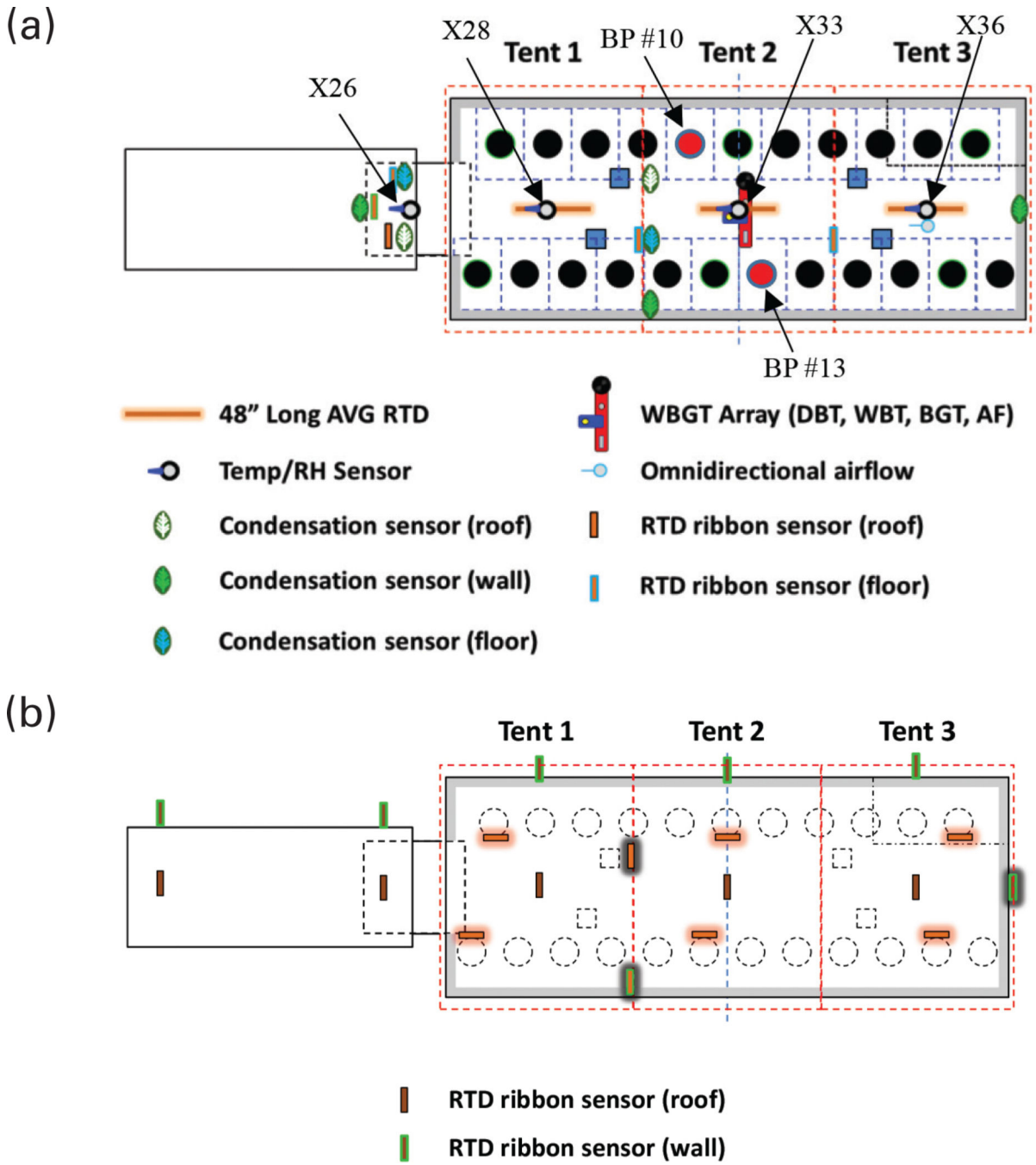
Figure 3. Sensor locations: (a) interior and (b) exterior.
