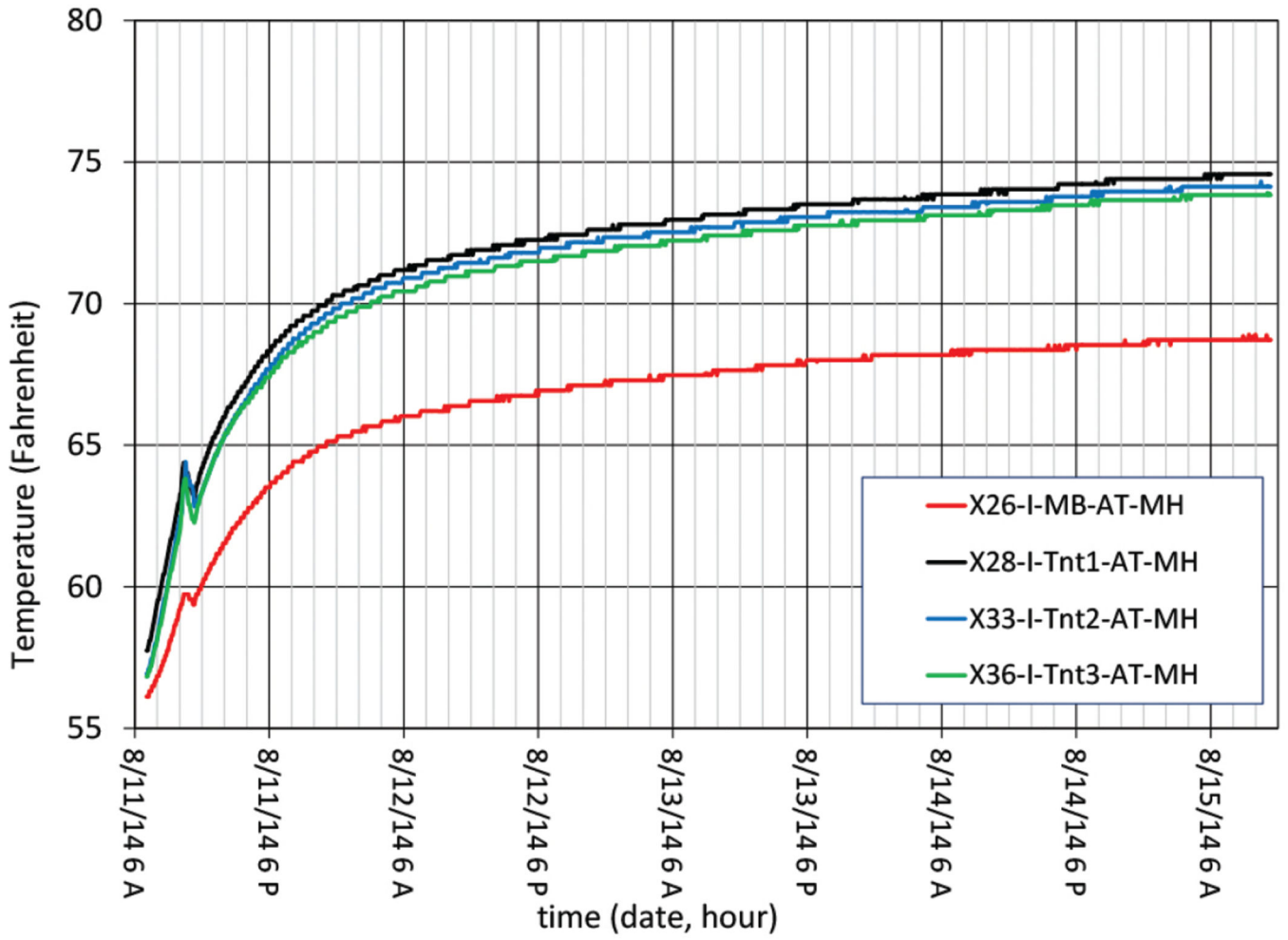
Figure 4. RA internal air temperatures at various locations.
