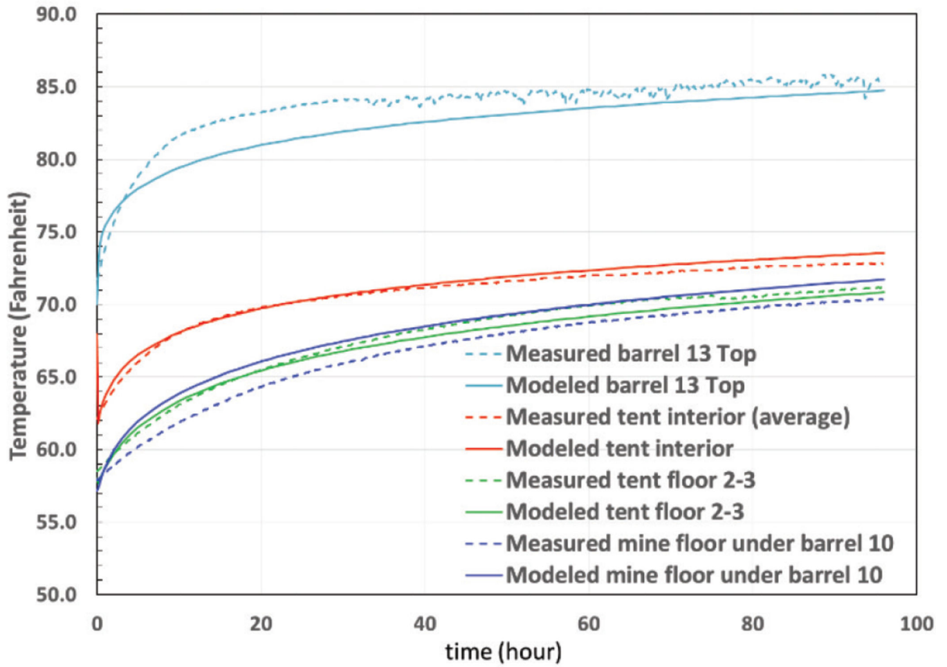
Figure 7. Simulated (solid line) versus measured (dotted line) temperature results for the top of the BP #13 simulated miner; the interior air at mid-height; the floor strata, underneath the intersection of Tent 2 and Tent 3, of the tested RA; and the mine floor under BP #10.
