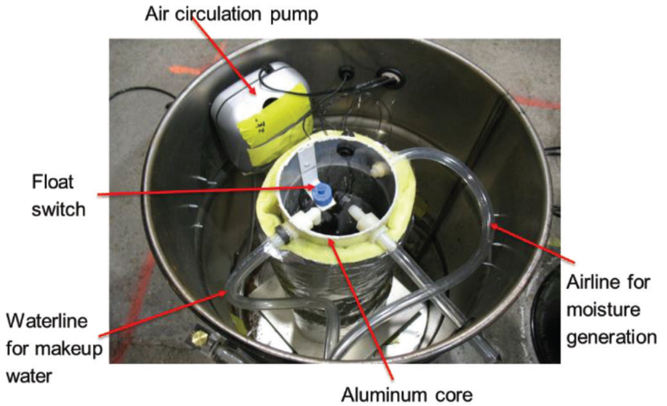
Figure 2. Inside view of a simulated miner.
