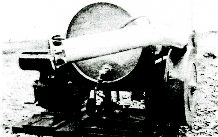
a - Close-up of centrifugal fan type sprayer.
