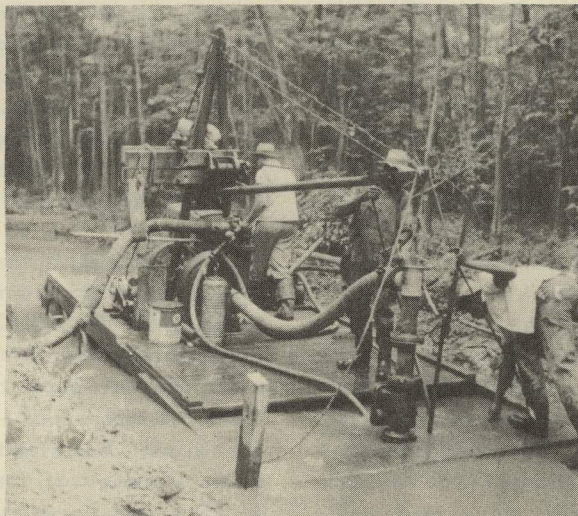
HYDRAULIC DREDGE
