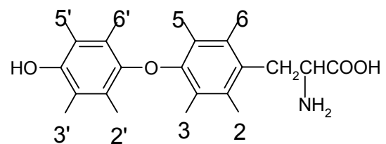
Thyronine
