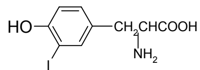
Iodotyrosine
