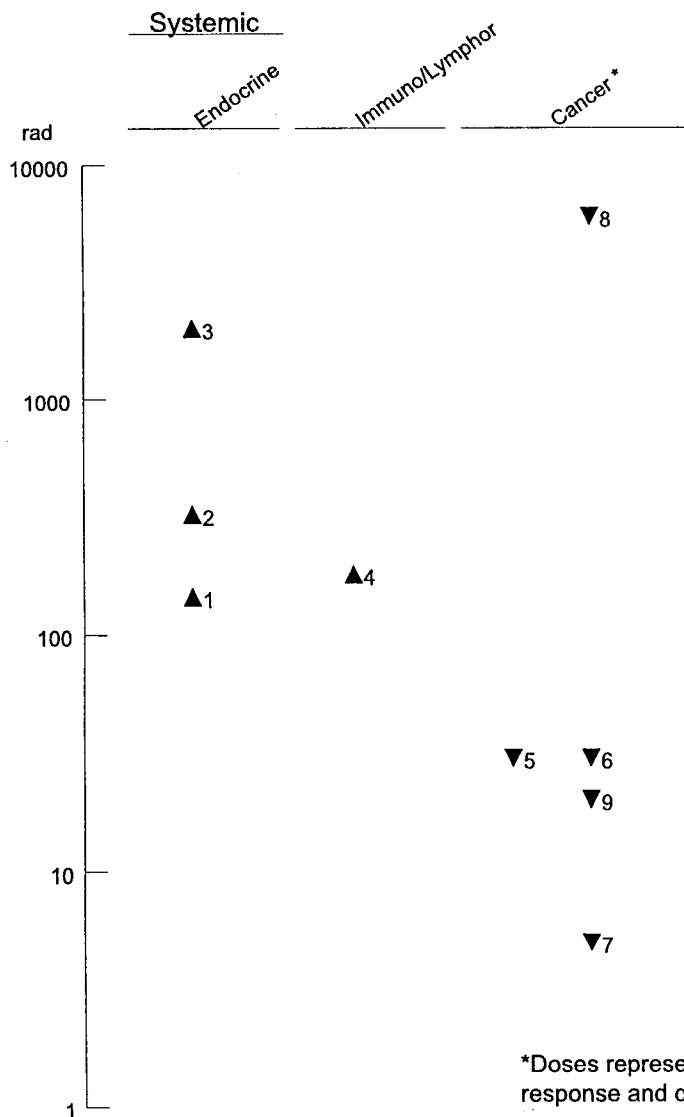
Figure 3-2. Levels of Significant Exposure to Iodine - Radiation Toxicity - Oral Acute ( \leq 14 days)
