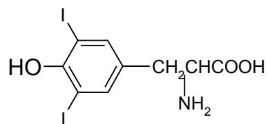
Diiodotyrosine
