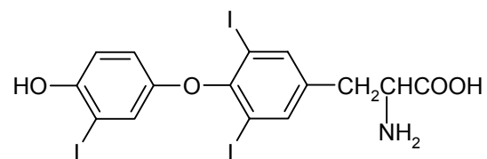
3,5,3'-Triiodothyronine (T 3 )
