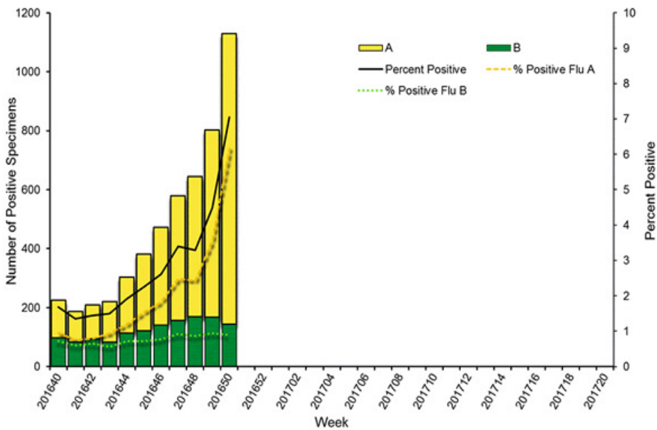
Influenza Positive Tests Reported to CDC by U.S. Clinical Laboratories, National Summary, 2016-2017 Season
