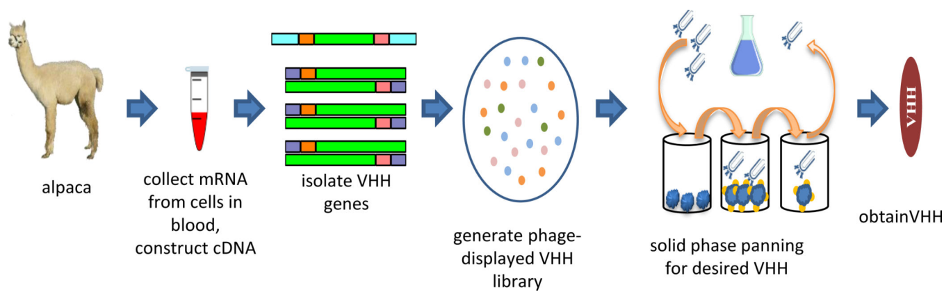
Figure 2. Overview of the process to isolate VHH from camelids. Briefly, mRNA is collected from the animal and converted into cDNA by RT-PCR. The cDNA is amplified and digested in order to isolate the VHH genes that are incorporated into plasmids and expressed by bacteriophage, creating a library. The library is panned for desired VHH.
