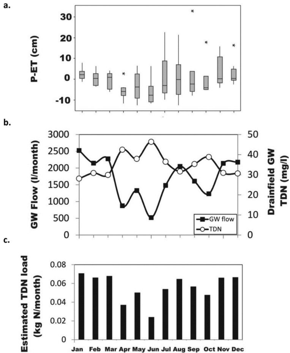
Fig. 8. (a) Monthly effective precipitation (precipitation-ET) at Plymouth, NC from 2004–2012. The boxplots display the 25 th to 75 th percentiles within the box; the median is indicated by the line inside the box. The whiskers extend to the upper and lower limits of the distribution, and asterisks indicate unusually large or small outliers. (b) Predicted monthly groundwater flow and drainfield groundwater TDN concentration. (c) Predicted monthly TDN load.
