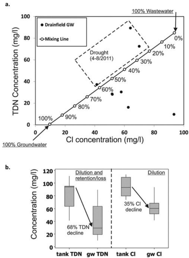
Figure 6. a. Chloride and TDN concentrations in drainfield groundwater plotted with 2-component mixing model line (components of wastewater and background groundwater). b. The boxplots display the 25 th to 75 th percentiles within the box; the median is indicated by the line inside the box. The whiskers extend to the upper and lower limits of the distribution, and asterisks indicate unusually large or small outliers. The boxplots show the declines in TDN and CL between the tank (wastewater) and drainfield groundwater.
