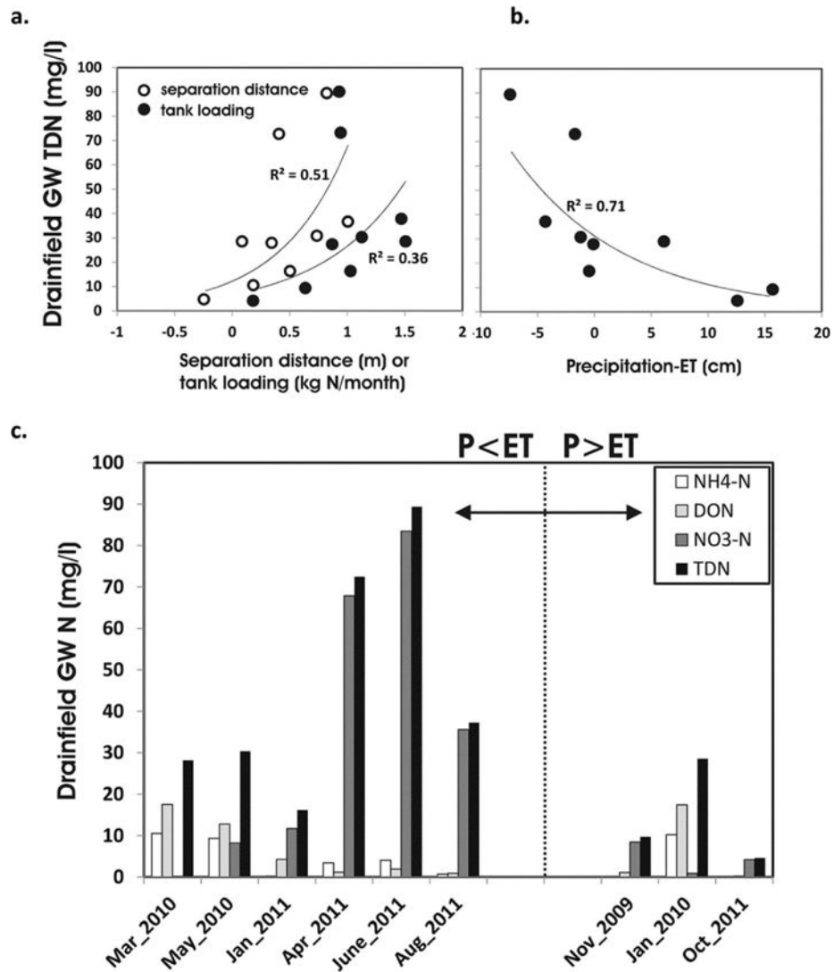
Figure 2. a. Separation distance (m) [ y = 12.147 e^{1.713x} ] or tank loading (kg-N/month) [ y = 6.722 e^{1.374x} ] versus the drainfield groundwater TDN concentrations. b. Effective precipitation (Precipitation-evapotranspiration (cm)) for two weeks prior to sampling versus the drainfield groundwater TDN concentrations [ y = 31.231 e^{-0.102x} ]. c. Drainfield groundwater nitrogen concentrations grouped by sampling dates during periods of precipitation deficits (P < ET) or precipitation excess (P > ET).
