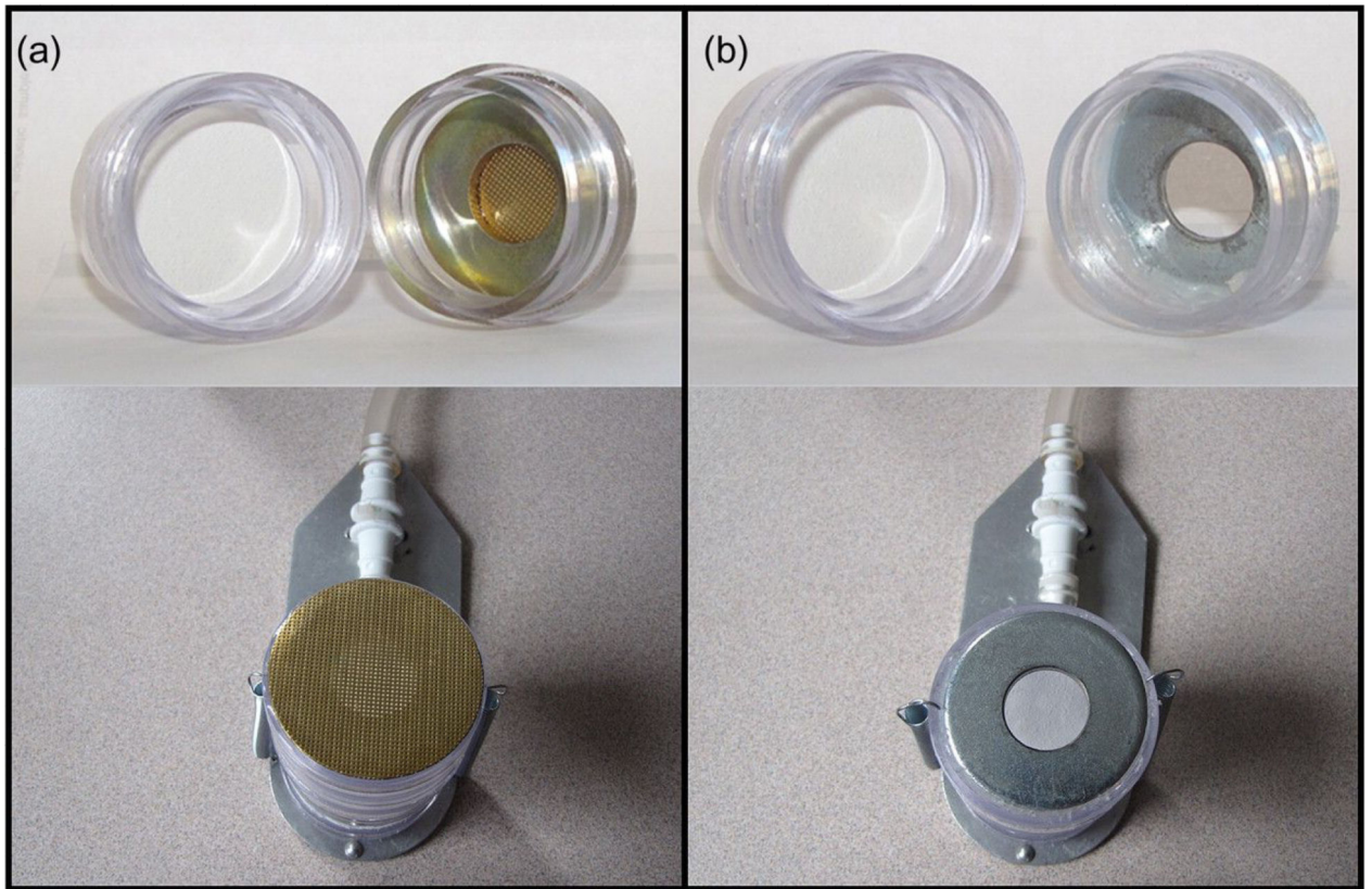
Fig. 1. (a) Photograph of constructed screened PHISH; (b) photograph of open-faced PHISH.
