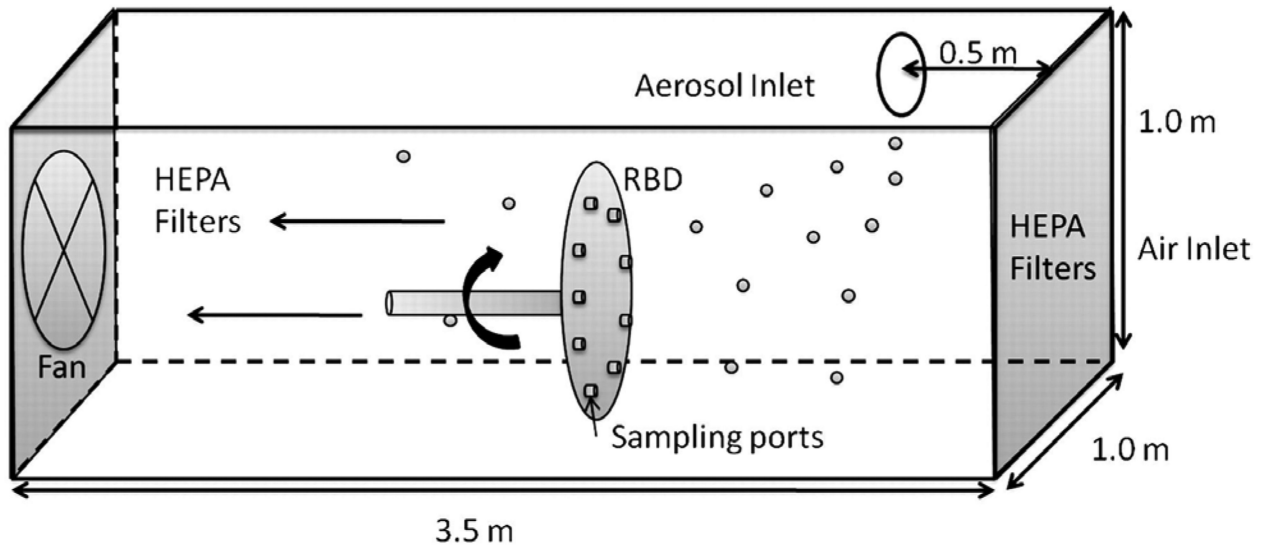
Fig. 2. Schematic of the wind tunnel showing aerosol inlet and location of the RBD.
