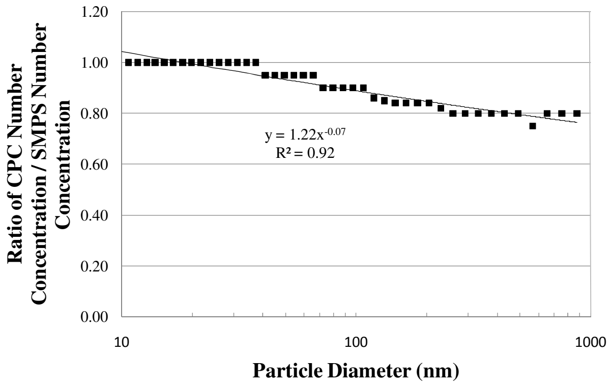
Supplementary Information Figure 1: Iterated DE values with the fit regression line.
