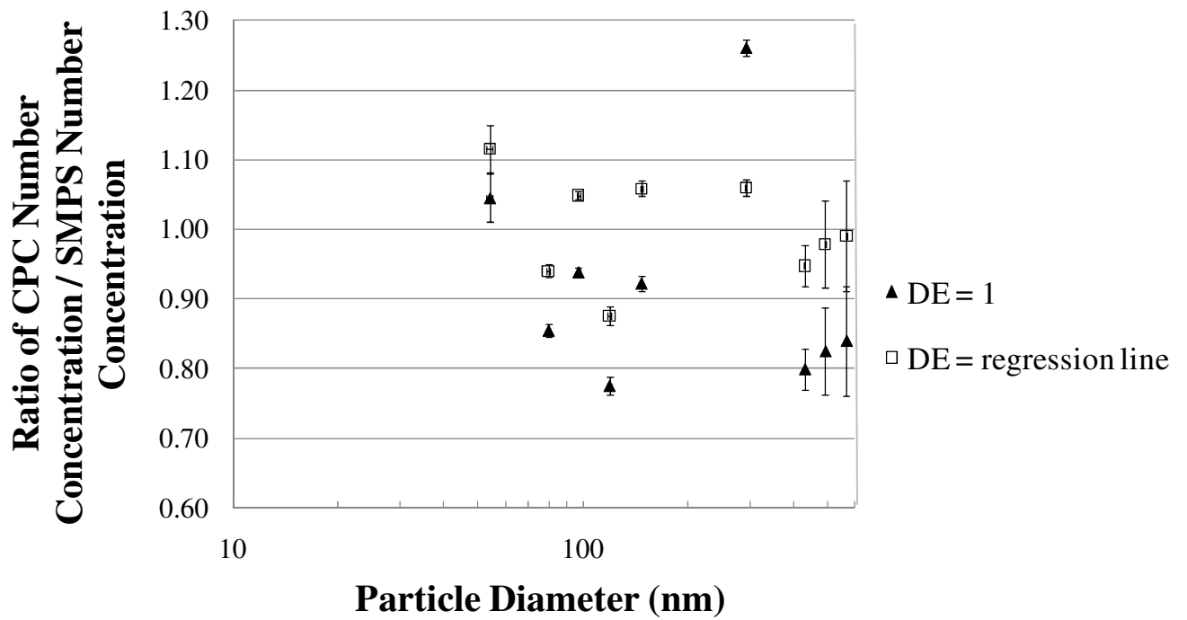
Supplementary Information Figure 2: Ratios of CPC number concentration to the product of SMPS number concentration and DE_d when DE_d values equaled 1 and when they equaled the regression line.
