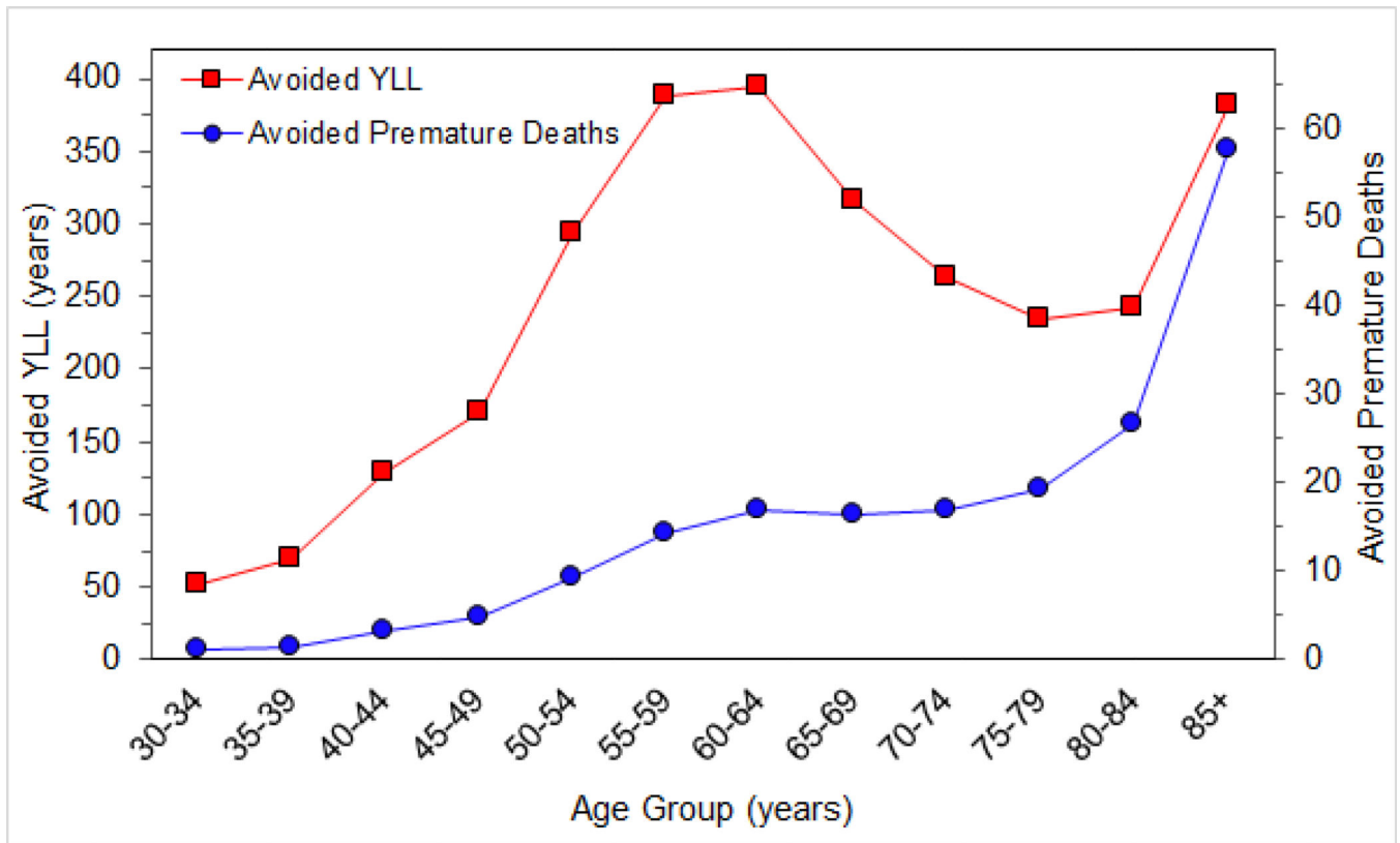
Figure 1. Number of avoided premature deaths and years of life lost (YLL) per year by age group in Wayne County for a reduction in PM 2.5 concentration from 10 to 8 µg/m 3 .
