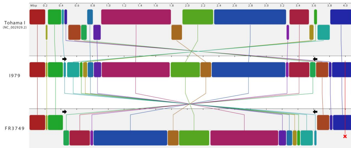
Technical Appendix Figure. Genomic rearrangement in Bordetella pertussis strains I979 and FR3749 compared with vaccine strain Tohama I, aligned in progressiveMauve ( http://darlinglab.org/mauve/user-guide/progressivemauve.html ). I979 and FR3749 differ by 1 large rearrangement. Location of the 28-kb deletion that includes the ptx/pta operon is marked by a red vertical line.
