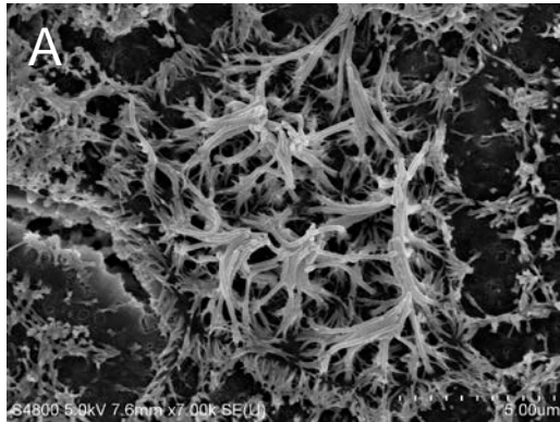
Naïve Control
