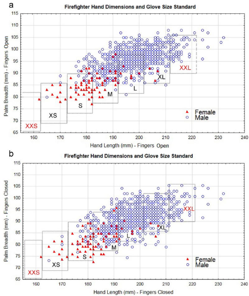
Figure 2. Matching firefighter hand dimensions with National Fire Protection Association 1971 glove-sizing scheme. (a) Data distribution in fingers-open posture. (b) Data distribution in fingers-closed posture. The rectangles represent the hand length and palm breadth ranges corresponding to the glove sizes.
