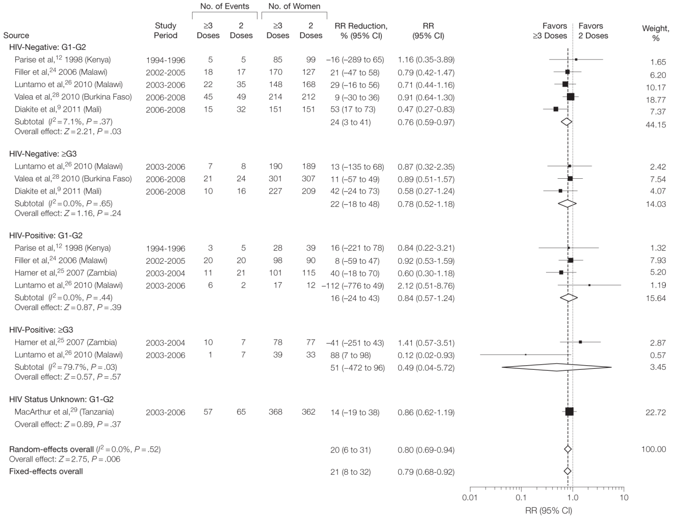
Figure 1. Meta-analysis of the Risk of Low Birth Weight in Trials Comparing the Standard 2-Dose vs 3 or More Doses of Intermittent Preventive Therapy During Pregnancy With Sulfadoxine-Pyrimethamine G1–G2 indicates first and second pregnancies; G3, 2 or more previous pregnancies; HIV, human immunodeficiency virus; RR, relative risk. P values after the I 2 statistics represent the \chi^2 test for heterogeneity. Dersimonian-Laird method used to calculate random-effects models; Mantel-Haenszel for fixed-effects models. Weights are from random-effects analysis. Data marker sizes indicate the weight applied to each study with random-effects meta-analysis. Test for subgroup differences: \chi^2_4=0.62 , P =.96, I 2 =0.0%.
