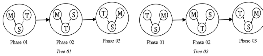
Figure 8. Two example trees showing the objective functions relationships in each phase
