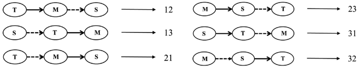
Figure 5. Description of different Chow-Liu trees generated using three variables ( T \rightarrow M = 1 ; M \rightarrow S = 2 ; S \rightarrow T = 3 )
