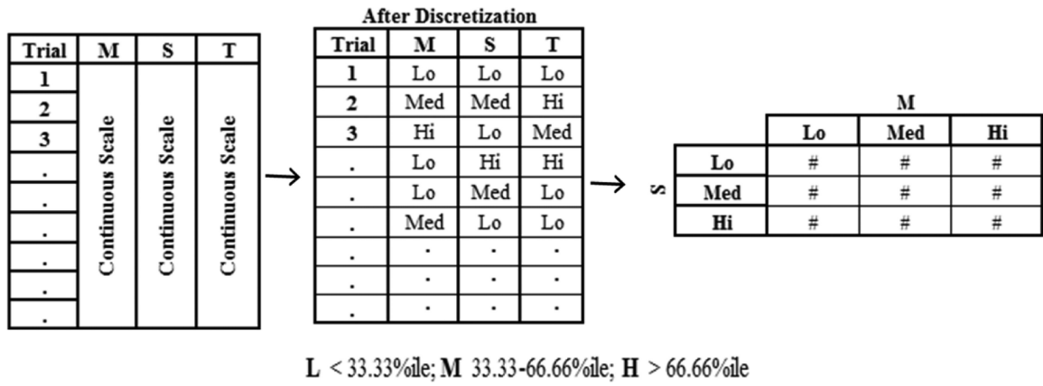
Figure 4. Flow chart showing steps involved in developing a condition probability table
