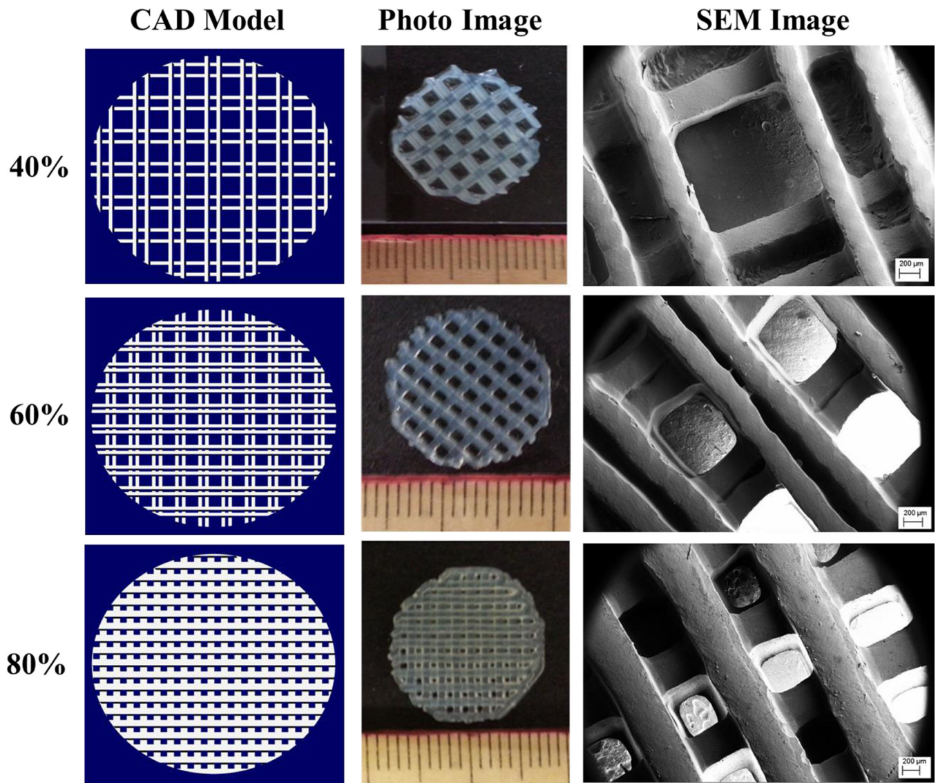
Figure 3. CAD models, optical, and scanning electron micrographs of hydrogel scaffolds with varying in-fill densities.
