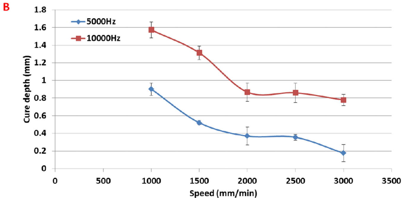
Figure 2. Optical micrograph (A) of cure depth samples at 5000 Hz and cure depth plot (B) of pulsed laser UV crosslinking of 60% PEG-Da/PEG (wt%) at 5000 Hz and 10000 Hz.
