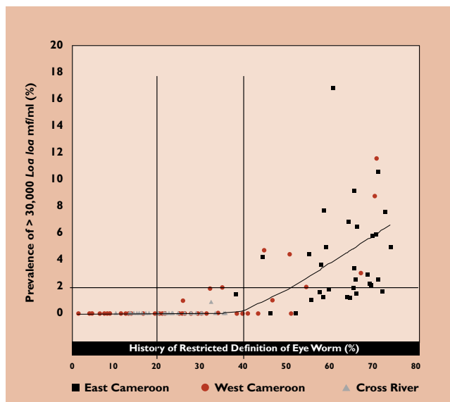
Figure 1 Prevalence of persons with L. loa microfilaria \geq 30,000 per ml as a function of the prevalence of a restricted definition of eyeworm, from Figure 10 of the multi-center report on RAPLOA [10]. See RAPLOA in the List of Abbreviations for details on the restricted definition of eyeworm.
