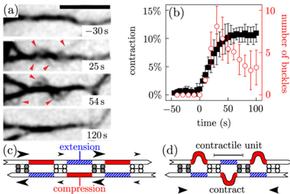
Fig. 2. Buckling in nonsarcomeric contractile actomyosin bundles. (a) Time-lapse images of fluorescent actin (inverted contrast) showing F-actin buckling (arrowheads) following the addition of 1 mM ATP at t = 0 s. Scale bar, 5 \mu\text{m} . See also movie S2 [18]. (b) Relative contraction (filled squares) and number of F-actin buckles (open circles) as a function of time. Data show mean \pm sd averaged over n = 3 bundles with \ell_0 \simeq 1 \mu\text{m} . (c) The presence of fast (gray) and slow (white) motors generically induce compressive (solid red) and extensile (hatched blue) stresses in filaments. (d) Buckling of the compressed filaments leads to an overall shortening of the bundle.
