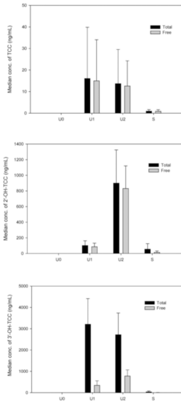
Figure 3. Median total and free concentrations of TCC (A), 2'-OH-TCC (B), and 3'-OH-TCC (C) from urine (U0, U1, and U2) and serum samples (S) collected from 9 rats dosed with 500 mg/kg body weight TCC. The error bars indicate the standard deviation of the measurements.
