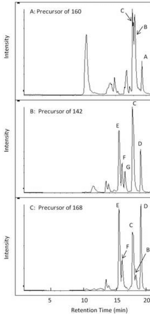
Figure 1. Total ion chromatograms of precursor ion scans (m/z 160, 142, and 168) from urine samples collected from nine rats after the administration of TCC.
