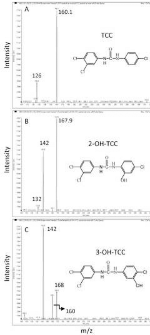
Figure 2. Enhanced product ion (EPI) mass spectra of different precursors in urine collected from rats after the administration of TCC: A) precursor A, B) precursor D, and C) precursor C.
