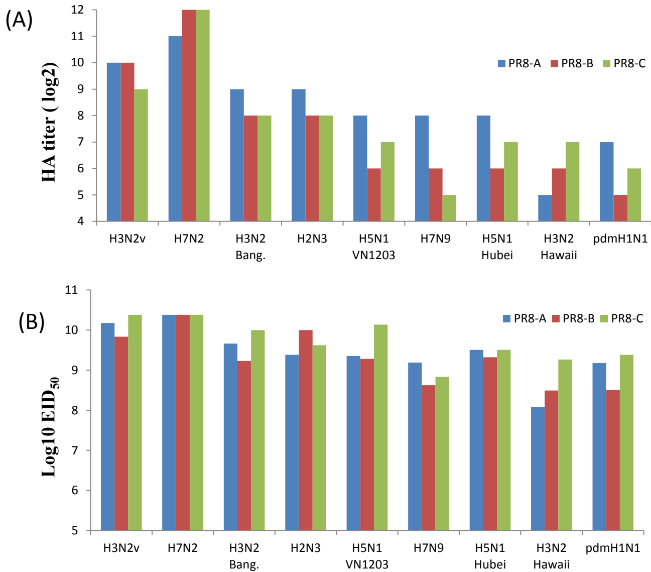
S1 Figure. Hemagglutination (A) and egg infectious titers (B) of reassortant viruses propagated in embryonated eggs.
