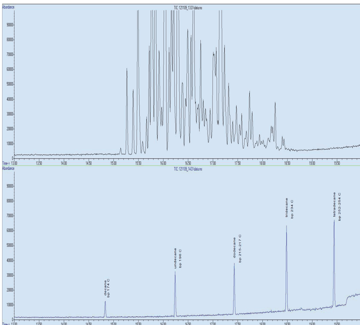
Figure 5. GC-MS chromatogram of DF-2000 diluted in methylene chloride.
