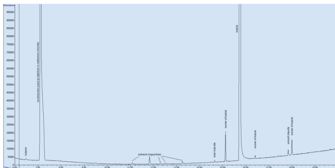
Figure 4. GC-MS chromatogram of SolvonK4 diluted in methylene chloride.
