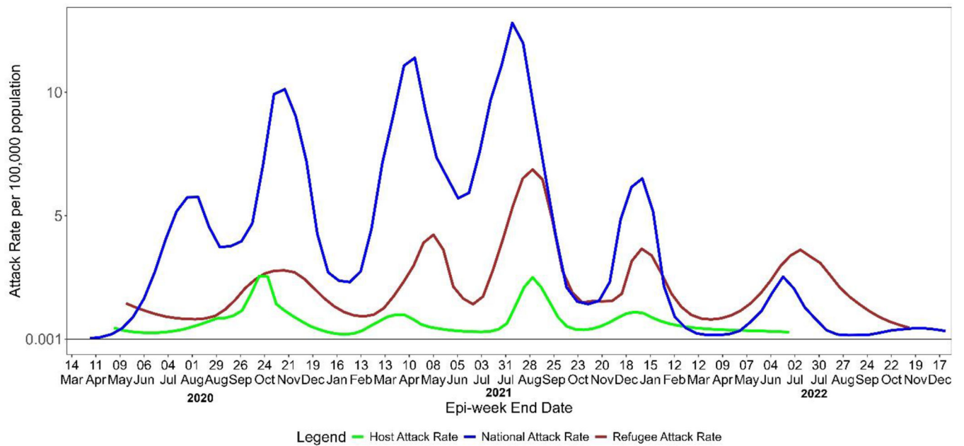
Figure 1: Weekly SARS-CoV-2 infection attack rates for Kenya, refugees and host population, March 12, 2020, to December 31, 2022.
