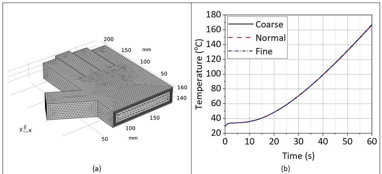
Figure 4. (a) Mesh structure in firefighters' gloves model created by free tetrahedral elements; (b) Mesh independence study on the 3D entire glove-hand model under high-heat condition (the temperature data were exported from Probe 5 – the hand skin surface temperature at the center of palm).
