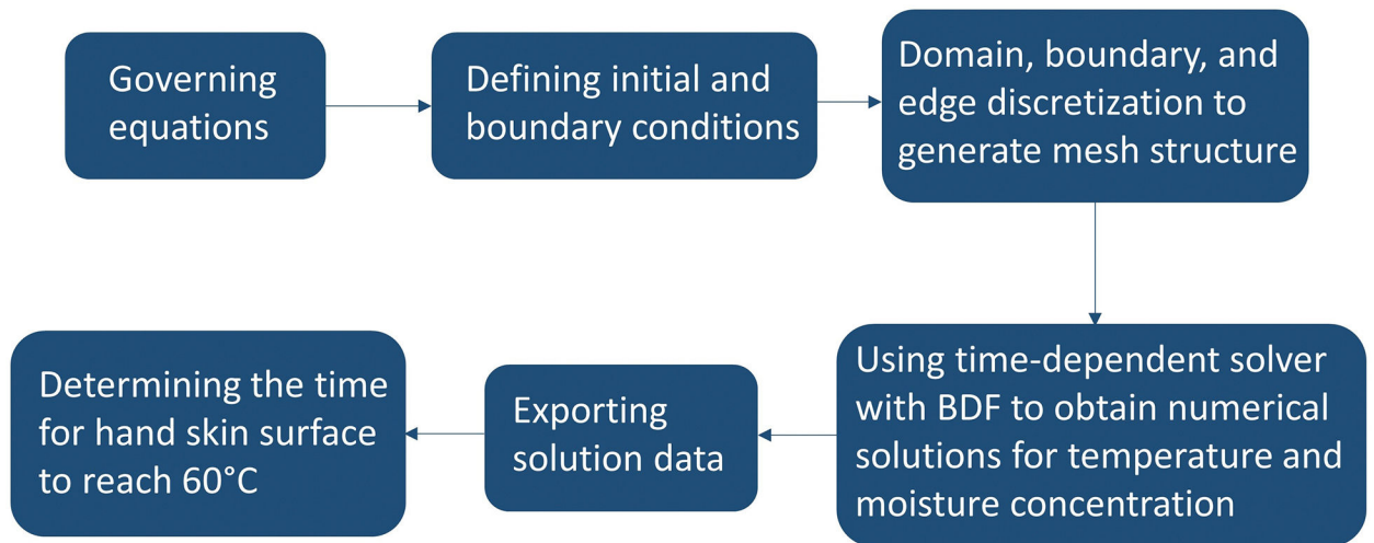
Figure 2. Flow chart for numerical solution procedure.
