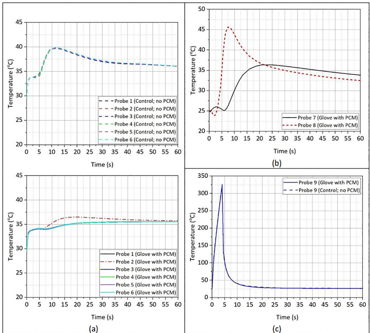
Figure 9. Temperature profiles at the (a) hand skin surface, (b) embedded PCM, and (c) glove outer surface during the cooling period after fire exposure, considering the effects of hand sweating, the moisture content in the environment, and external water spray from a hose. The glove was cooled with water spray.
