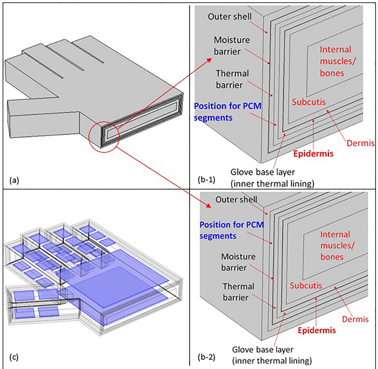
Figure 1. Geometry of the 3D glove-hand model: (a) Overall view of the 3D glove-hand model; (b-1) and (b-2) each glove and skin layer in the model (b-1: PCM located ABL in glove, b-2: PCM located BOS in glove); (c) the positions of PCM segments in the glove (blue parts indicate PCM segments). Air gaps existed between each glove layer as well as between hand and glove in the simulation model.
