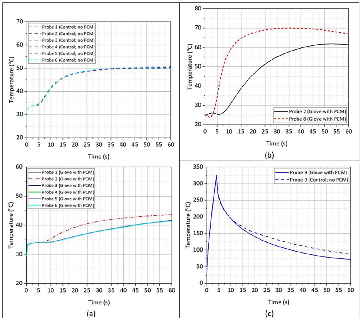
Figure 8. Temperature profiles at the (a) hand skin surface, (b) embedded PCM, and (c) glove outer surface during the cooling period after fire exposure, considering the effects of hand sweating and moisture content in the environment. The glove was cooled by ambient air only.
