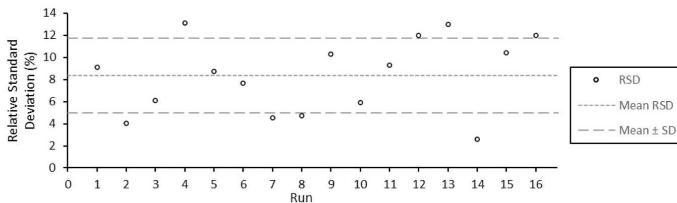
Figure 5. The plot of intra-run RSD of the percent recovery of n-heptane from solid sorbent samplers ( n = 4 ) collected from 16 runs of generated atmospheres of 0.1 ppmv 10 VOC mixture. The mean (short dashes) plus/minus the standard deviation (long dashes) of the intra-run RSDs are shown.
