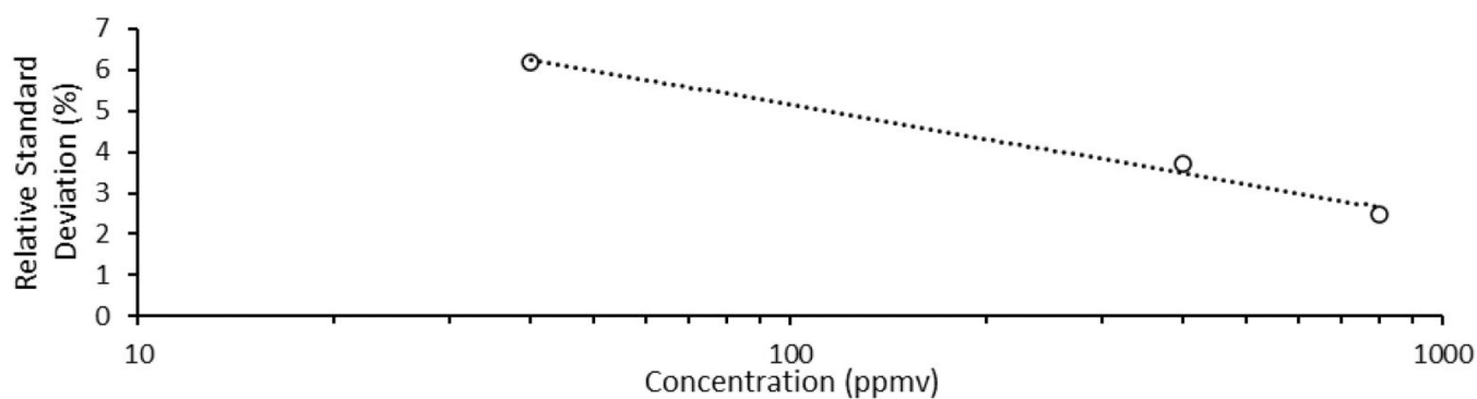
Figure 3. Relative standard deviation of the intra-run mean ( n = 6 samplers) percentage recovery of n-heptane in the generated atmosphere versus target concentration plotted with the concentration axis in log scale.
