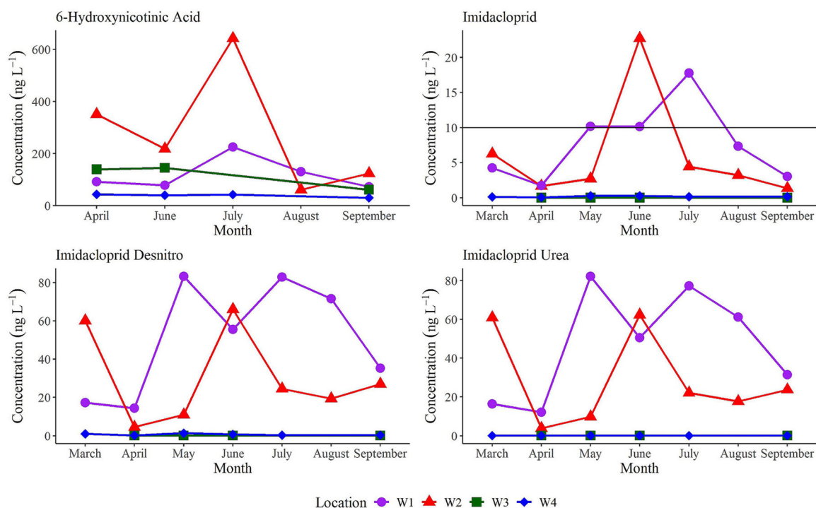
Fig. 5. POCIS-derived estimated concentrations of imidacloprid and its by-product over the study period for each site. The horizontal black line denotes the EPA's aquatic life benchmark for the chronic toxicity limit for freshwater invertebrates of 10 ng L -1 for imidacloprid (EPA, 2023a).
