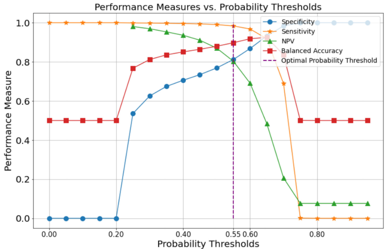
Fig. 2. Performance measures associated with different probability thresholds for non-wear classification. The optimal probability threshold (.55) was selected since, at this probability, the best tradeoff between NPV and specificity was achieved.
