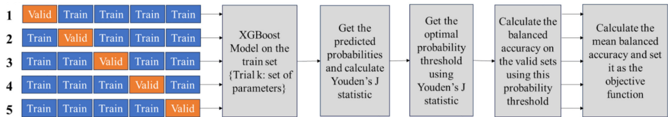
Fig. 1. Hyperparameter tuning and k-fold cross-validation to optimize XGBoost model parameters.
