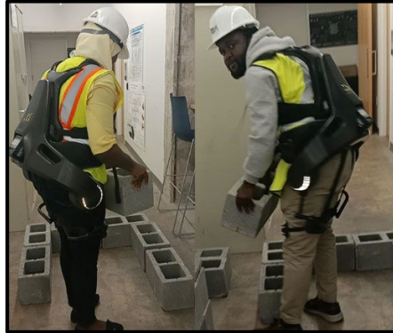
Fig 1: Active Exoskeleton
