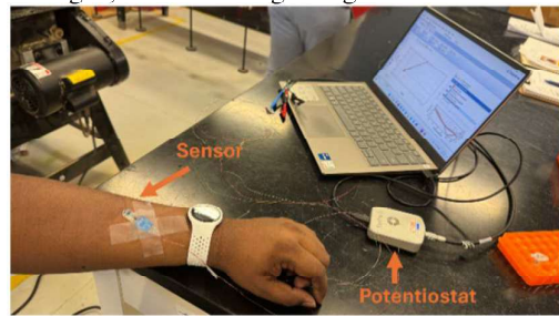
Fig. 2. Schematic representation of sensor mounted on the forearm and data acquisition with the EmStat4S potentiostat.
