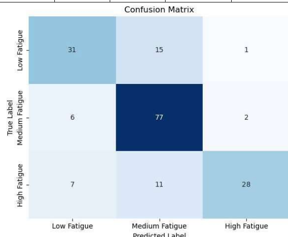
Fig. 4. Confusion matrix for the SVM classifier.
